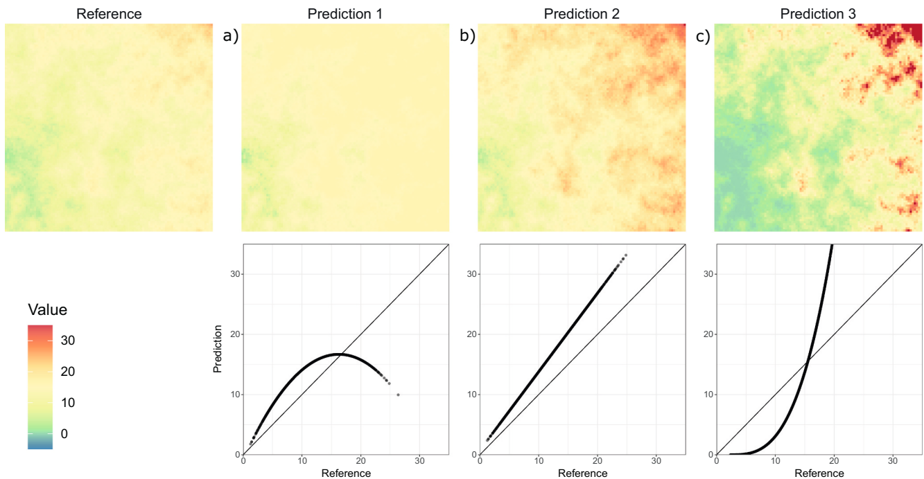
Fig. 1. A reference map with three modifications of this map taken as prediction. Predictions 1 has predicted values \hat{z}_1 = -0.82 + 2.15z - 0.07z^2 , where z is the value from the reference map. Prediction 2 is obtained with \hat{z}_2 = 0.74 + 1.31z and prediction 3 with \hat{z}_3 = 0.007(z - 2.248)^3 . The three prediction maps have the exact same level of agreement (i.e. \rho_c = 0.6 ) with the reference map.
