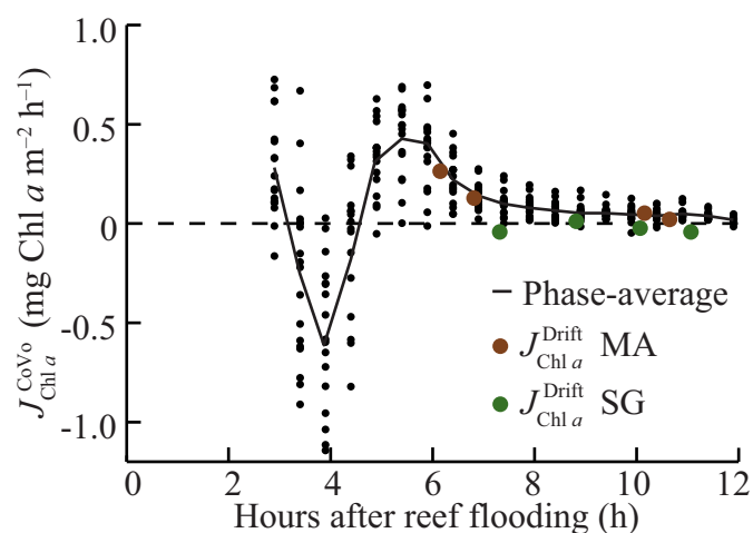
Fig. 6. All estimates of benthic flux of Chl a using the one-dimensional control volume technique ( J_{\text{CoVo}}^{\text{Chl } a} ). Positive values indicate net uptake by the reef and negative values indicate net release to overlying waters. Individual estimates (black dots) shown with tidal phase-averaged flux (line) and flux estimates from drifter releases ( J_{\text{Chl } a}^{\text{Drift}} ) in macroalgal (MA) and seagrass (SG)-dominated zones.
