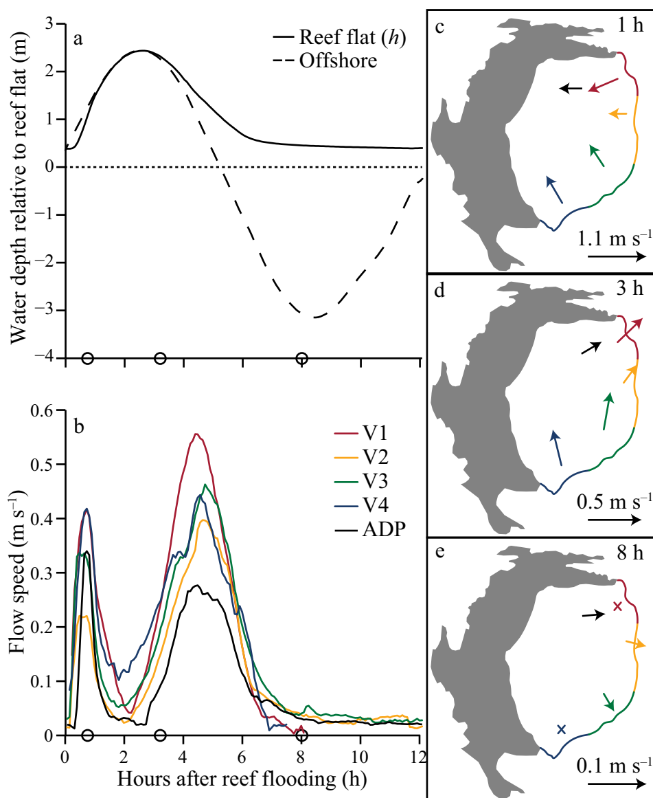
Fig. 2. Tidal phase-averaged hydrodynamic conditions on Tallon Reef including (a) water depth at SG ( h ) and offshore; (b) current speed at five hydrodynamic instruments (V1–V4 are acoustic Doppler velocimeters and ADP is an acoustic Doppler profiler); and current vectors from (c) flood tide, (d) start of ebb tide, and (e) middle of ebb tide. All values are means from a full spring-neap cycle. Note scale changes on current vectors to emphasize flow patterns. Crosses indicate periods when water depth was too low to measure flow. Length of reef crest ( l_r ) used for discharge estimates (see “Methods” section) is colored to correspond with associated hydrodynamic instrumentation.
