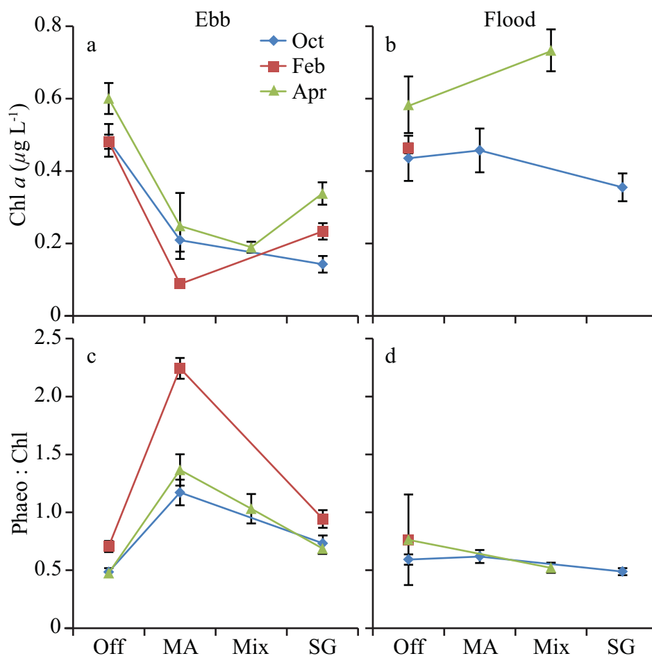
Fig. 3. Mean ( \pm SE) Chl a ( a , b ) and ratio of phaeopigments : Chl a ( c , d ) from water samples at offshore (Off) and reef stations [macroalgal (MA), mixed (Mix), and seagrass (SG) dominated zones] during all field experiments. Samples are categorized as taken during flood tide or during ebb tide (final 6 h) on the reef platform. The number of samples represented by each mean is shown in Table 1. [Color figure can be viewed at wileyonlinelibrary.com ]
