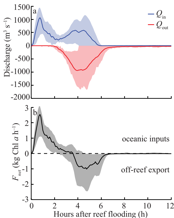
Fig. 7. Tidal phase-averaged (lines) and ranges (shaded areas) of (a) discharge and (b) net rate of Chl a transfer F_{\text{net}} onto (positive) and off of (negative) Tallon reef platform are shown with hours after reef flooding. Discharges are onto ( Q_{\text{in}} ) and off of ( Q_{\text{out}} ) the reef platform. [Color figure can be viewed at wileyonlinelibrary.com]
