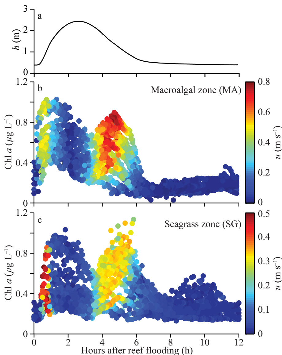
Fig. 5. Reef flat (a) depth h (tidal phase-averaged) shown with all Chl a measurements from fluorimeters in (b) macroalgal and (c) seagrass-dominated zones shown with hour after reef flooding during the Apr field experiment. Color indicates the flow speed u adjacent to each fluorometer. Note that different limits are used in the color scale of each plot in order to accommodate differences in the range of flow speeds at each station.
