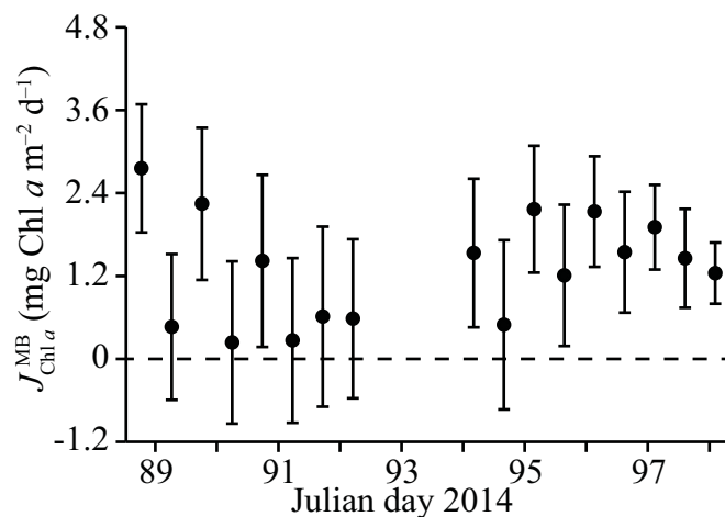
Fig. 8. Mean ( \pm SD) vertical flux of Chl a over each tidal cycle determined by the mass balance technique ( J_{\text{Chl } a}^{\text{MB}} ) for the Apr field experiment. Positive values indicate net uptake of Chl a on the reef platform, while negative values indicate net release of Chl a to the overlying waters.
