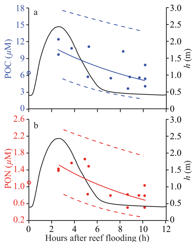
Fig. 9. Concentrations of particulate organic (a) carbon (POC) and (b) nitrogen (PON) on the reef (station Mix) during the Apr field experiment, shown as a function of hours after reef flooding. Mean tidal phase-averaged water depth h shown in black. Colored lines, which indicate the relationship between POC and PON with time after reef flooding ( R^2 = 0.46 and 0.57 , respectively), were used to estimate nutrient concentration in off-reef discharge during ebb tide. Dashed lines represent 95% confidence limits of the mean. Colored circles on the x-axis denote mean concentration offshore.
