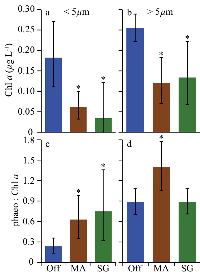
Fig. 4. Mean (with 95% confidence limits) Chl a concentration ( a, b ) and ratio of phaeophytin : Chl a ( c, d ) from water samples in small ( < 5 \mu\text{m} ) and large ( > 5 \mu\text{m} ) fractions at offshore (Off) and reef stations [macroalgal (MA) and seagrass (SG) dominated zones]. All samples taken during the Oct field experiment during final 6 h of ebb tide on the reef (Table 1). Asterisks (*) denote means which are significantly different ( p < 0.05 ) to offshore means. [Color figure can be viewed at wileyonlinelibrary.com ]
