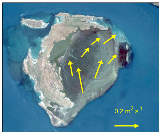
Figure 7. Residual discharge \langle \vec{q} \rangle computed for the duration of the experiment.
