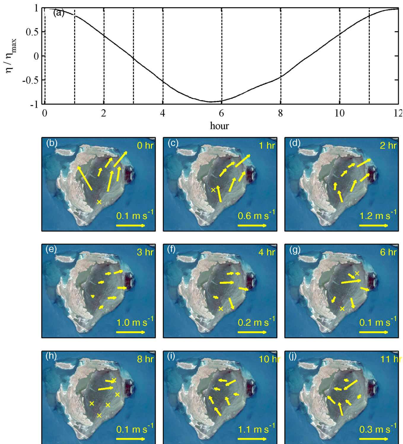
Figure 6. Tidal current vector fields on the reef at select phases of the tide. (a) For reference, the tidal phase-averaged offshore water level at P1, normalized by the mean tidal range. Vertical-dotted lines denote the select phases of the tide plotted in Figure 6b–6j. Tidal phase-averaged current vectors at select phases of the tide, referenced to the time of peak high tide ( t=0 ); (b) 0 h; (c) 1 h; (d) 2 h; (e) 3 h; (f) 4 h; (g) 6 h; (h) 8 h; (i) 10 h; and (j) 11 h. Note that the current vectors are scaled substantially among figures to emphasize the current patterns when the flow is relatively weak (refer to the reference current vector for scaling differences). The “x” symbols represent either flow speeds <0.01 \text{ m s}^{-1} or when the water was too shallow to measure flow.
