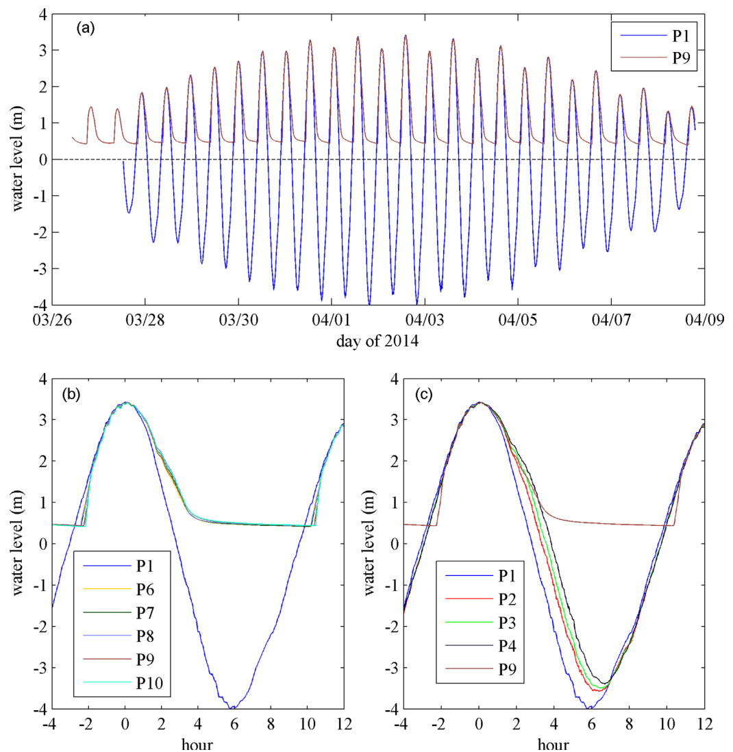
Figure 4. Water level variability. (a) Water level variations at a representative site offshore (P1) and on the reef platform (P9) for the entire experiment. For a single tidal cycle on 2 April, (b) the water levels measured at all pressure sensor sites on the reef (P6–P10) relative to offshore (P1), and (c) measured at all offshore sites (P1–P4) relative to on the reef (P9). Note that in Figures 4b and 4c time is defined relative to peak high tide when t = 0 h.
