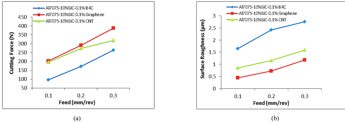
Fig. 3.(a),(b).The effect of feed rate on cutting force and surface roughness at cutting speed 90 m/min and depth of cut 1.5 mm using DLC coated carbide tool.
