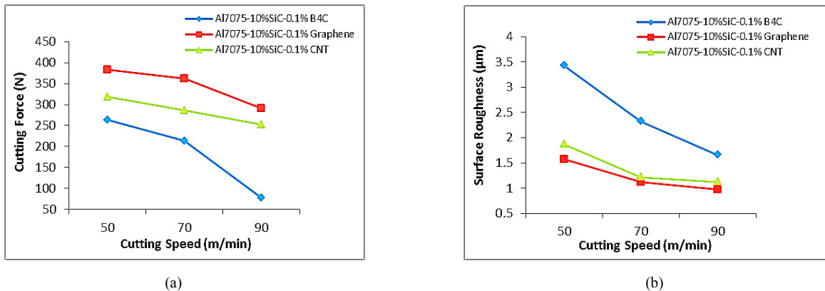
Fig. 2. (a),(b) The effect of cutting speed on cutting force and surface roughness at feed rate 0.3 mm/rev and depth of cut 1.5 mm using DLC coated carbide tool.
