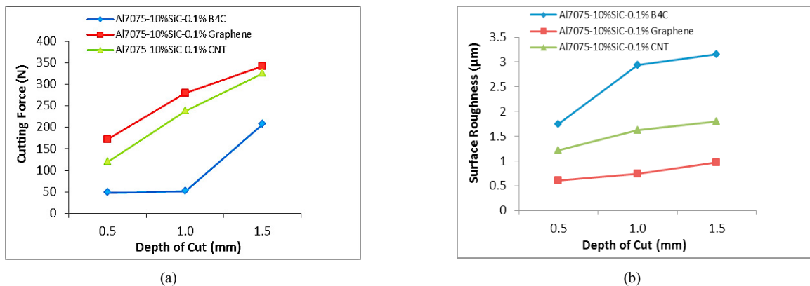
Fig. 4.(a),(b) The effect of depth of cut on cutting force and surface roughness at cutting speed 90 m/min and feed rate 0.3 mm/rev using DLC coated carbide tool.
