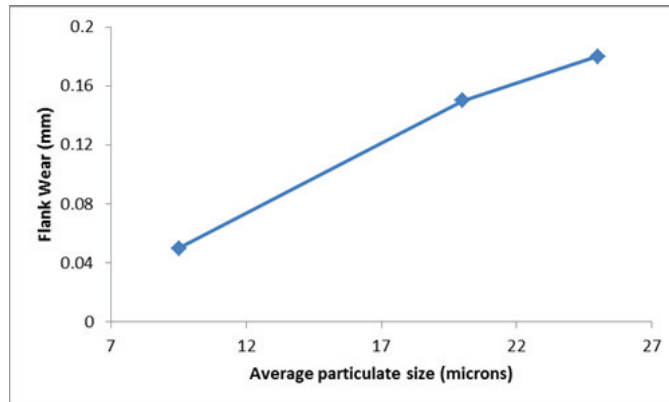
Fig.1. Flank wear during machining of Al 6061/10% \text{Al}_2\text{O}_3 composite with various particles size [14]
