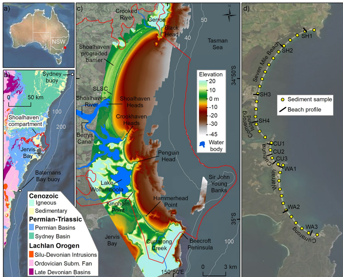
Fig. 1 A Study site location on the NSW coast. B Simplified geology showing location of the secondary level Shoalhaven Coastal Compartment (red outline) and Sydney and Batemans Bay wave-rider buoy. Isobaths in metres. C Combined topographic and marine
