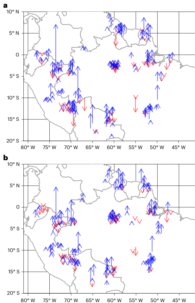
Fig. 2 | Spatial trends of mean tree size and the scale parameter across Amazonian forests. a, b. Distribution of annual trends of mean tree BA (a) and scale parameter (b) per inventory plot across Amazonia. Trends represent the slope of a linear regression fit to mean tree size and scale parameter within each inventory plot. These vary from -7.1 \times 10^{-4} to 2.2 \times 10^{-3} \text{ m}^2 \text{ yr}^{-1} and -1.1 to 3.7 \text{ yr}^{-1} for mean tree size and scale parameter, respectively. Mean tree size changed on average by 1.45 \times 10^{-4} \text{ m}^2 \text{ yr}^{-1} across all plots, 3.3% gain per decade compared to initial mean size of 4.78 \times 10^{-2} \text{ m}^2 . The average change in scale parameter was 0.4 \text{ yr}^{-1} , 3.8% per decade compared to initial mean scale parameter of 103. Arrows show the magnitude and direction of trends at each plot location, with blue arrows showing increasing trends and red arrows showing declining trends.
