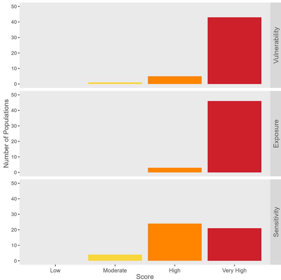
Fig. 2. Distribution of vulnerability, exposure, and sensitivity categories for all sea turtle units assessed.
