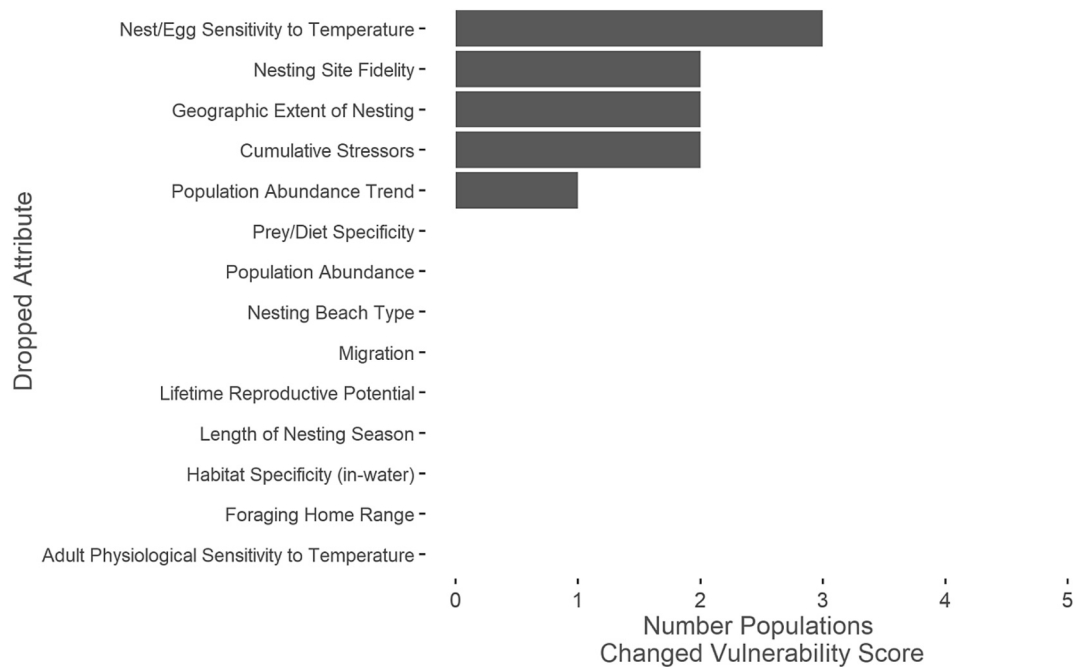
Fig. 6. Leave-one-out sensitivity analysis showing how many sea turtle units changed climate vulnerability score when a given sensitivity attribute was omitted.
