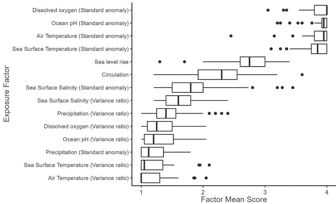
Fig. 3. Exposure factor mean scores for all sea turtle units assessed. The vertical bar represents the median; the box is bounded by the first and third quartiles; whiskers represent 1.5 times the inter-quartile range; points represent all outlying values.
