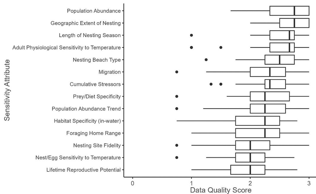
Fig. 12. Mean data quality score for each sensitivity attribute across all sea turtle units assessed. The vertical bar represents the median; the box is bounded by the first and third quartiles; whiskers represent 1.5 times the inter-quartile range; points represent all outlying values.
