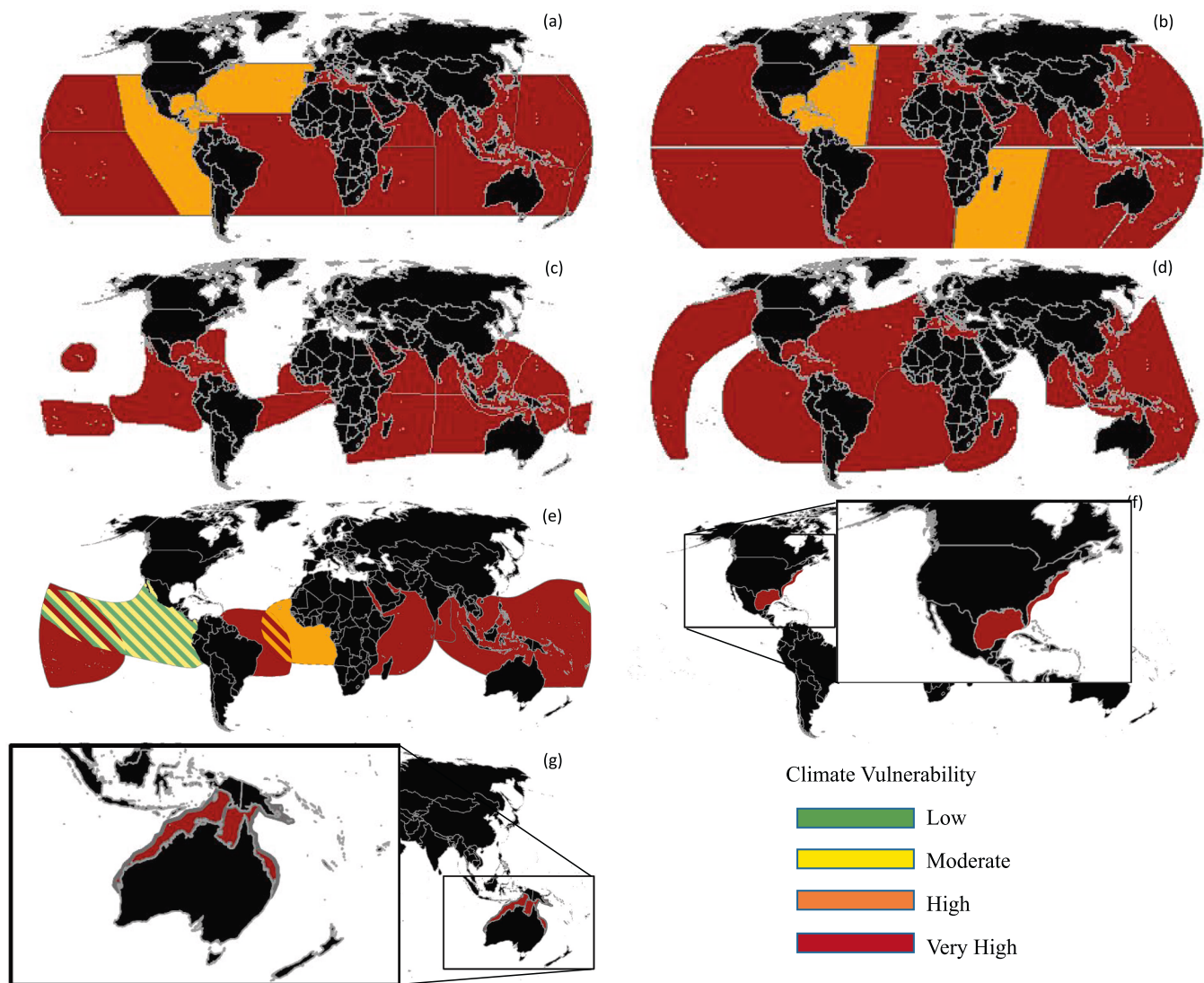
Fig. 8. Map of unit vulnerability by species. RMUs defined by Wallace et al. (2010, 2023); DPSs defined under the ESA (US 50 CFR § 223.102, US 50 CFR § 224.101). (a) green turtle ( Chelonia mydas ), (b) loggerhead ( Caretta caretta ), (c) hawksbill ( Eretmochelys imbricata ), (d) leatherback ( Dermochelys coriacea ), (e) olive ridley ( Lepidochelys olivacea ), (f) Kemp's ridley ( Lepidochelys kempii ), and (g) flatback ( Natator depressus ). (For interpretation of the references to color in this figure legend, the reader is referred to the web version of this article.)
