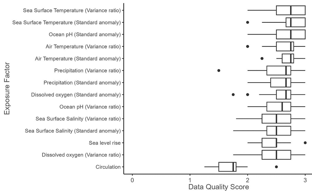
Fig. 11. Mean data quality score for each exposure factor across all sea turtle units assessed. The vertical bar represents the median; the box is bounded by the first and third quartiles; whiskers represent 1.5 times the inter-quartile range; points represent all outlying values.
