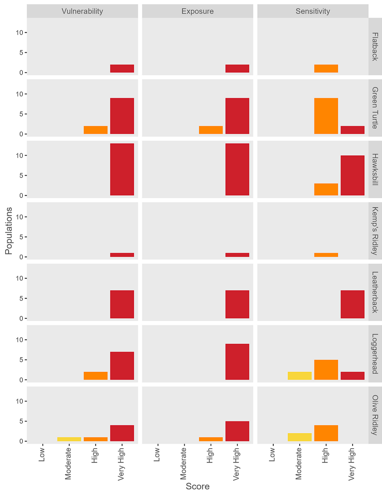
Fig. 9. Vulnerability, exposure, and sensitivity scores for each sea turtle unit by species.
