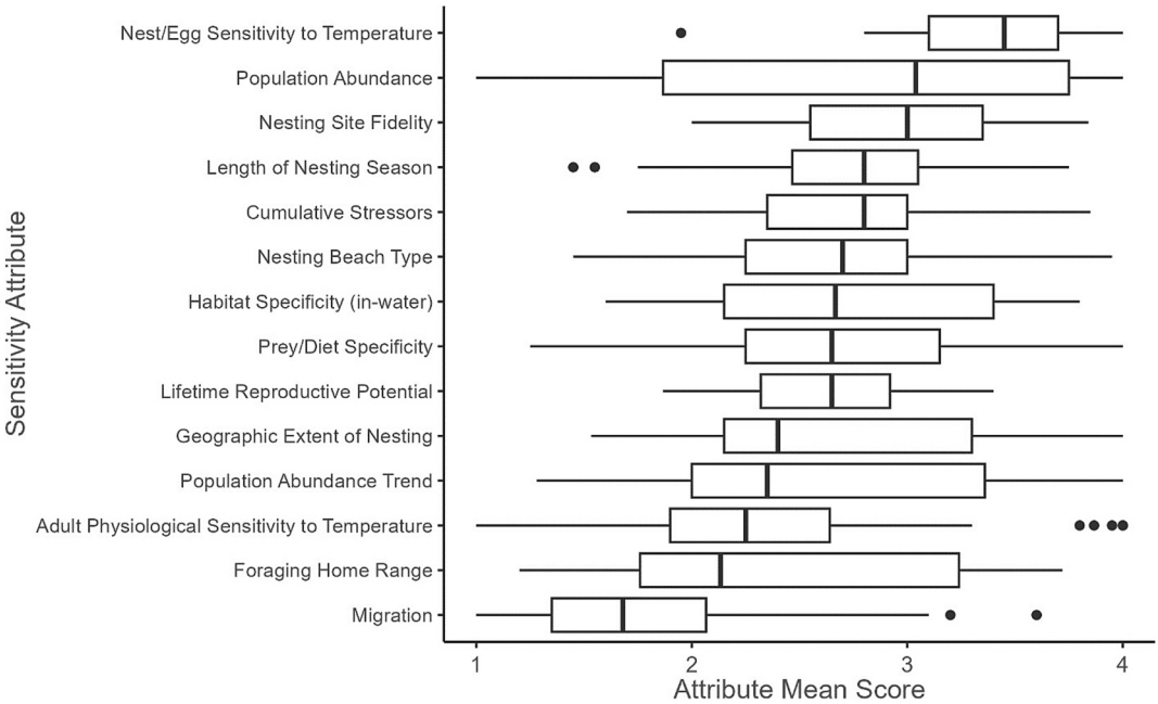
Fig. 5. Sensitivity attribute mean scores for all sea turtle units assessed. The vertical bar represents the median; the box is bounded by the first and third quartiles; whiskers represent 1.5 times the inter-quartile range; points represent all outlying values.
