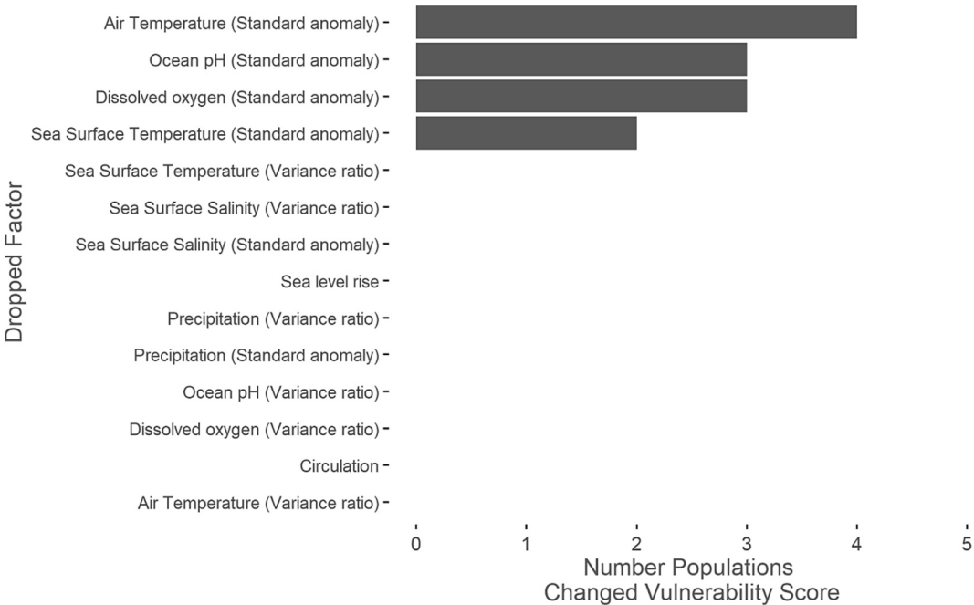
Fig. 4. Leave-one-out sensitivity analysis showing how many sea turtle units changed climate vulnerability score when a given exposure factor was omitted.
