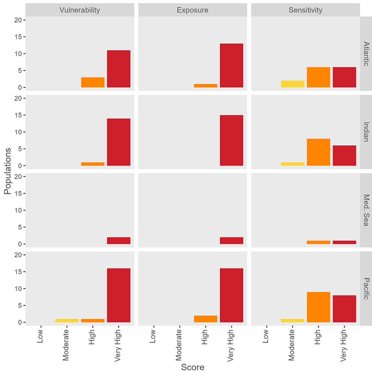
Fig. 10. Vulnerability, exposure, and sensitivity scores of each sea turtle unit by geographic region.
