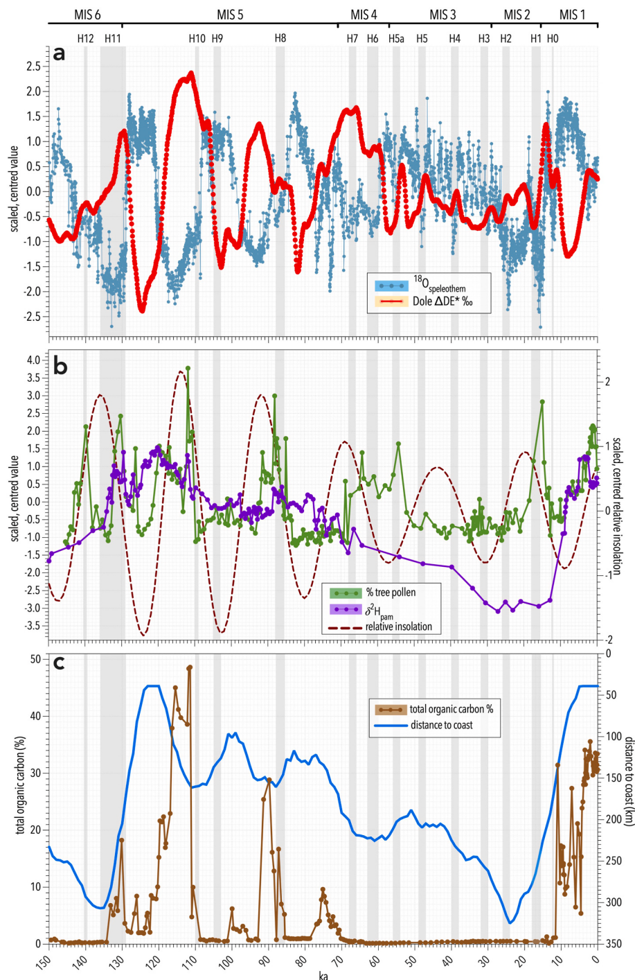
Fig. 2. (a) Composite east Asian summer monsoon speleothem oxygen isotope record (Cheng et al., 2016) and the Dole effect ( \Delta DE^* ) record (Huang et al., 2020). (b) \delta^2H_{pam} (hydrogen isotope composition of plant available moisture) and %tree pollen of total dryland pollen records from Girraween Lagoon summer (January–February–March) insolation at 18^\circ S ; all values are scaled and centred for correlation (see Methods, and extended data Figs. S2 and S3 for unscaled time series in original units with analytical errors). (c) Total organic carbon record from Girraween Lagoon and distance to coast (Bird et al., 2024). The timing of Heinrich events is indicated as grey shading and Marine Isotope Stage boundaries also shown, both from Lisieki and Stern (2016). The age of 140 ka for ‘H12’ in Lisieki and Stern (2016) is derived from the average age of two events centred on 135.5 ka and 144.3 ka (with no duration given for either event) identified by Channell et al. (2012), so ‘H12’ is likely of longer duration than shown above.
