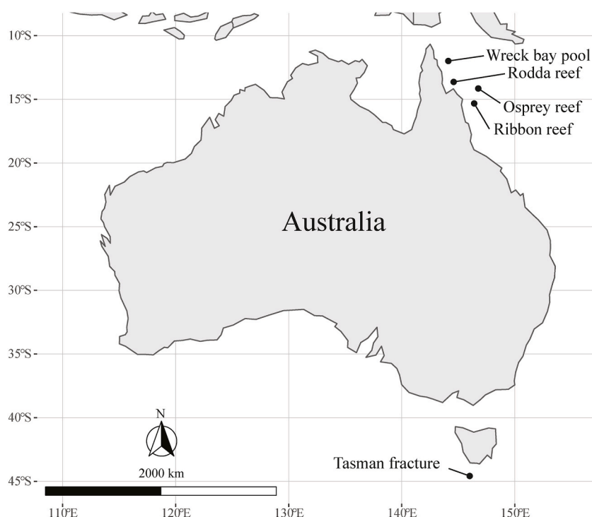
Fig. 1. Map showing the sampling location of the cold and deep sea water corals analyzed in this project.
