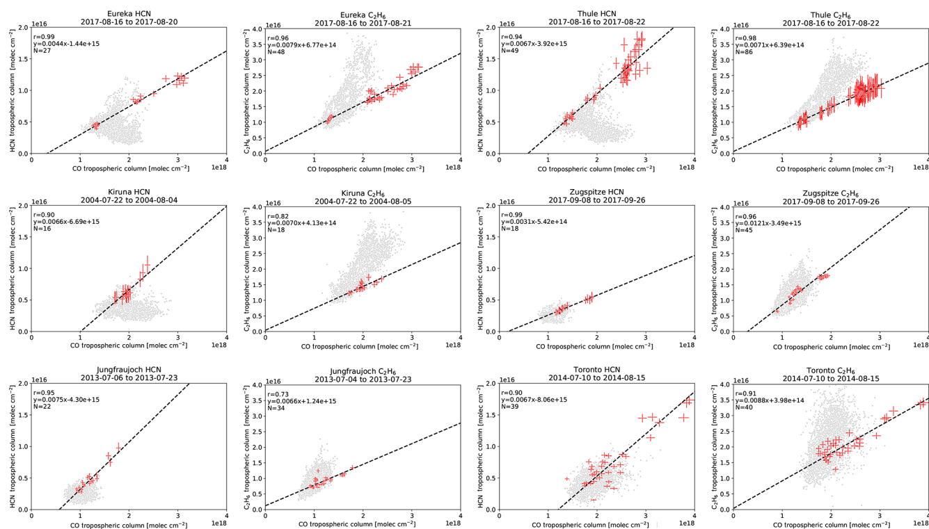
Figure A5. Examples of the enhancement ratios of HCN and C_2H_6 for a selected BONA wildfire pollution event at each site. The grey points indicate all years of measurements. The red points are measurements taken during the fire-affected period stated in the subplot title. The dashed black line is the linear regression to the red points. The number of measurements ( N ), linear equation, and correlation coefficient ( r ) are also shown.
