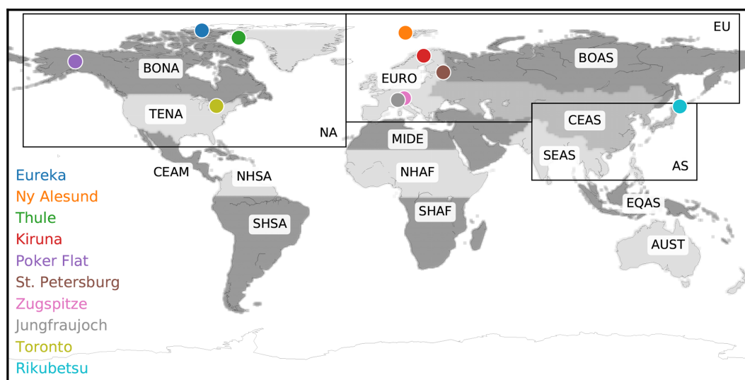
Figure 1. Locations of ground-based FTIR sites used in this study. The biomass burning regions (shaded) and anthropogenic source regions (black rectangles) used for the GEOS-Chem tagged CO simulation are also shown and summarized in Table 2.
