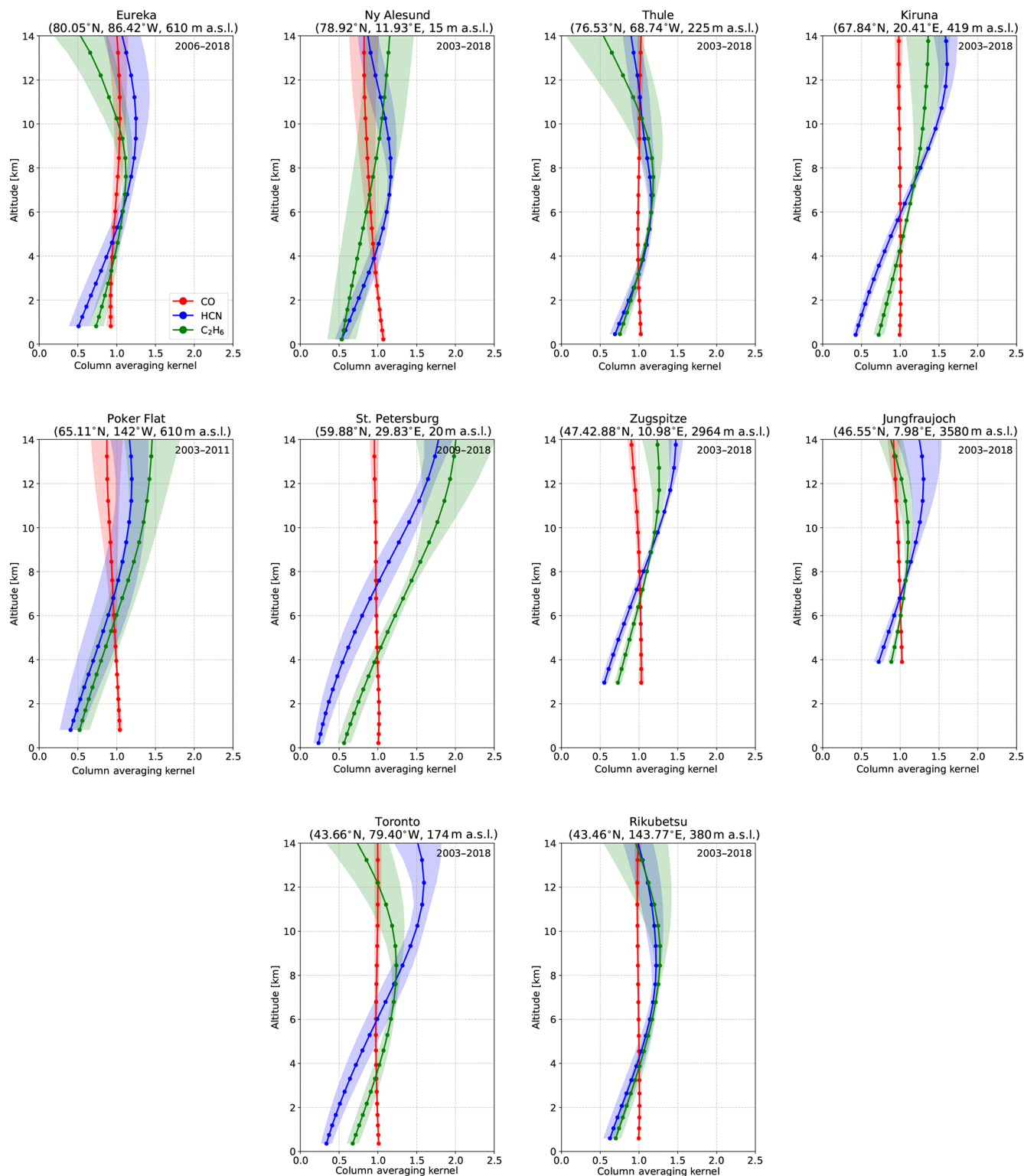
Figure A4. Mean CO, HCN, and C 2 H 6 normalized total column averaging kernels (molec. cm −2 /molec. cm −2 ), taken over all years of measurements at each site. The shaded region indicates a 1σ standard deviation from the mean. The circle markers indicate the layer centers of the FTIR vertical retrieval grid.
