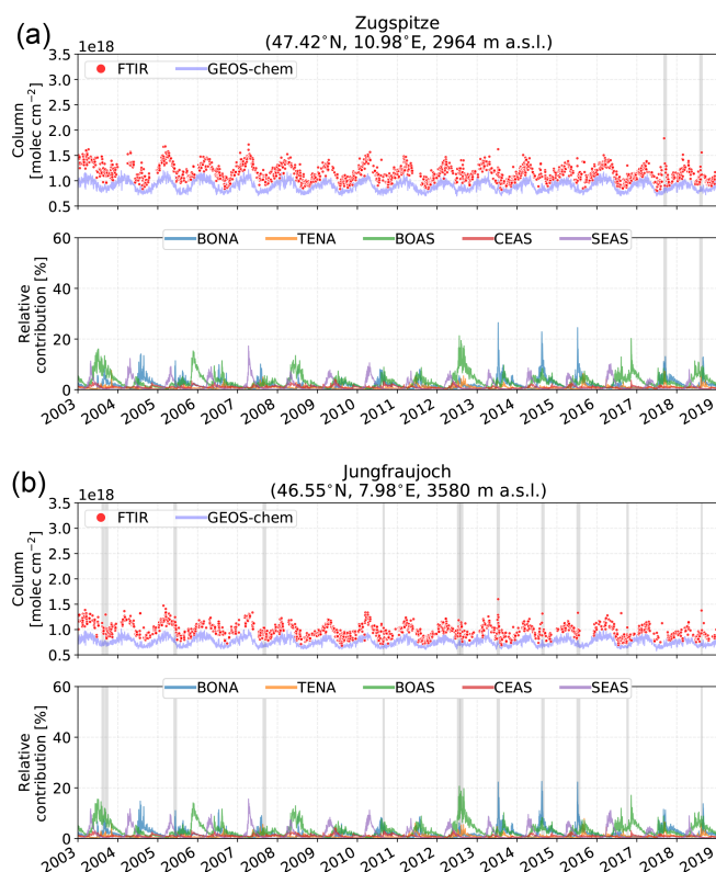
Figure 9. Same as Fig. 7 but for the Alpine sites: (a) Zugspitze and (b) Jungfraujoch.
