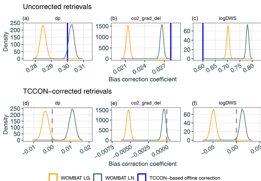
Figure 7. Posterior densities of bias-correction coefficients from inversions using OCO-2 retrievals without bias corrections applied (a, b, c) and those from inversions using retrievals corrected using the TCCON-based offline bias coefficients (d, e, f). Densities are shown for inversions based on LG and LN retrievals in yellow and dark green, respectively. The TCCON-based offline bias correction coefficients are shown as vertical blue lines for the panels in the top row. The vertical dashed grey lines in the bottom row mark zero, which is the value the coefficients would take if the data were unbiased.
