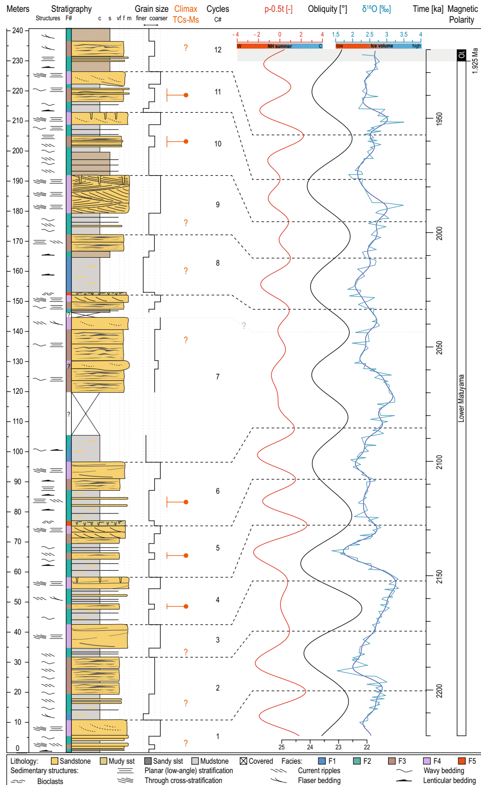
Figure 3. Stratigraphy and chronology of the lower Cholan Fm along the Houloung River. The stratigraphic data (facies, lithology, grain size) are compared and correlated to: (1) a mix-standardized precession minus 0.5 times standardized obliquity ( p-0.5t ) 39 as orbital reference based on the Laskar, et al. 7 solution (red curve), (2) pure obliquity curve (black curve) 7 , and (3) a \delta^{18}\text{O} record from benthic foraminifera (light blue curve) 40 smoothed (dark blue curve) using a Taner 41 low-pass filter with a cutoff frequency of 0.1 and a roll-off rate of 10^{10} using the 'astrochron' R package 42,43 . Climax periods of tropical cyclone and monsoon are pointed out by orange dots or orange "?". W: warmer, C: colder. The illustration was made using Adobe Illustrator CS6 ( https://www.adobe.com/ ).
