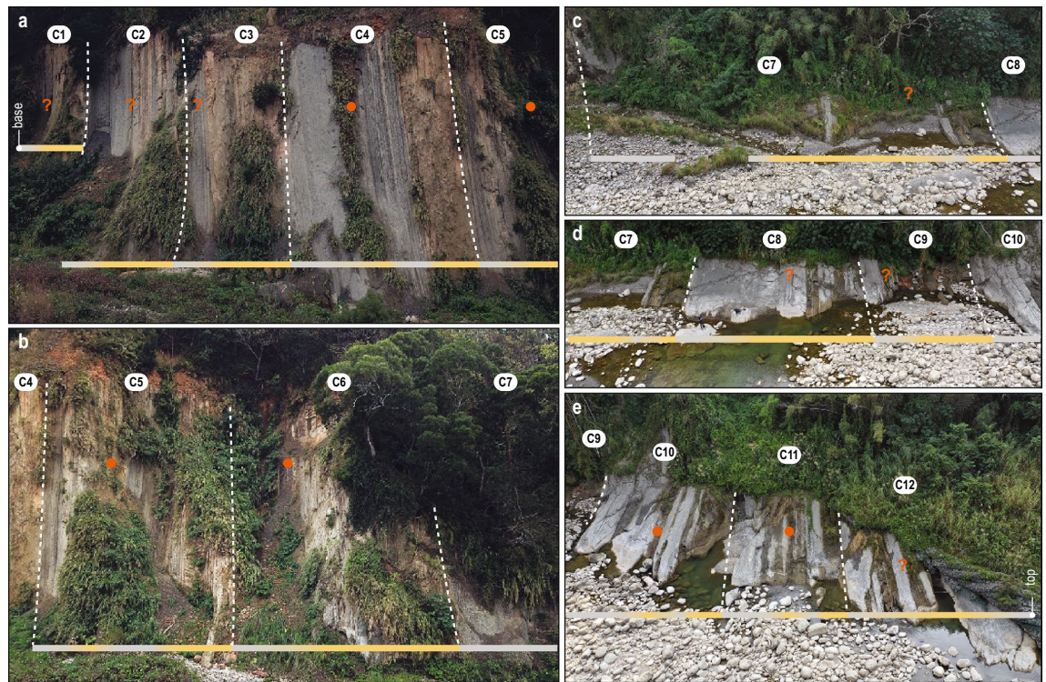
Figure 2. Drone footage of the lower Cholan Fm along the Houlong River (Fig. 1). Twelve cycles (C1–C12) are defined for the 241 m thick section, evolving from mudstone-prone to sandstone-prone sedimentary facies. Color scale bar: light gray: mudstone-prone, yellowish: sandstone-prone. Orange dots (and question marks) mark the climax of interactions between tropical cyclones and the monsoon, which are expressed as sandstone-prone heterolithics intervals. The illustration was made using Adobe Photoshop CS6 and Adobe Illustrator CS6 ( https://www.adobe.com/ ).
