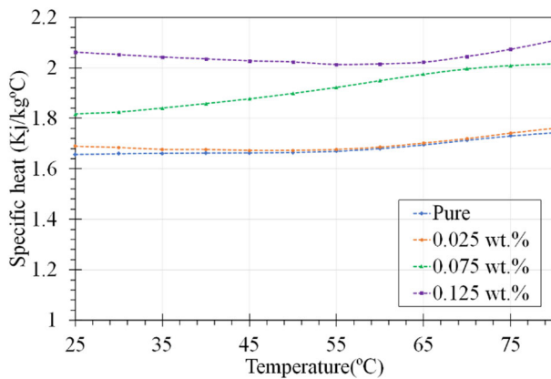
FIGURE 2. c_p variation of Soybean oil and SO/Ti 3 C 2 NFs at increasing temperature.
