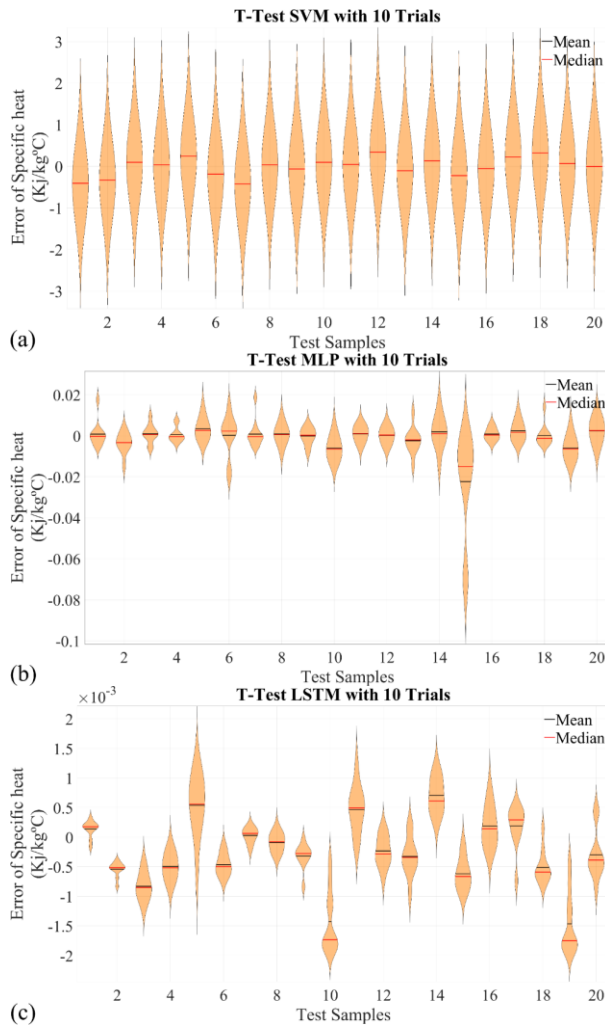
FIGURE 7. The results of the T-test after 10-time trials for proposed optimized machine learning methods, including (a): SVM; (b): MLP; (c): LSTM.
