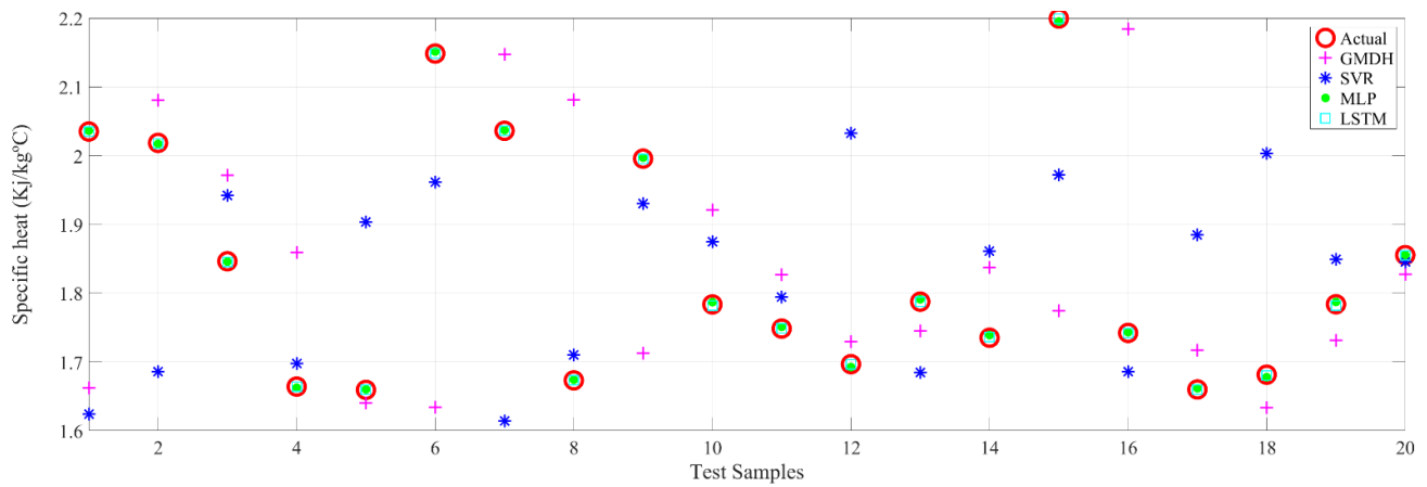
FIGURE 3. The actual and predicted c_{pNF} of soybean oil/MXene NFs based on temperature and nanoflake concentration using Bayesian optimization-based GMDH, SVR, MLP and LSTM machine learning methods.
