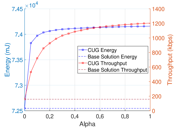
FIGURE 7. Throughput and energy consumption of the upload group with different values of \alpha .
