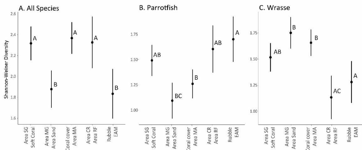
Figure 5. Shannon–Weiner diversity estimates (fitted values with 95% confidence intervals) in the habitat cluster for (A) all species, (B) parrotfish, and (C) wrasse. Letters adjacent to points are significance groupings based on post hoc multiple comparisons Tukey’s tests.
