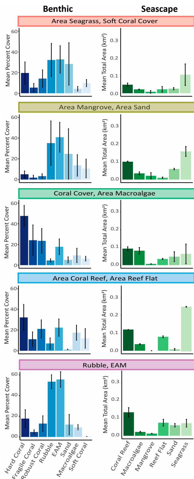
Figure 3. Average (mean) and variation (standard deviation) of percent cover or area of seascape variables (km 2 ) within each habitat cluster. The left column (blue) is the mean percent cover of benthic coral reef habitat variables observed on coral reef transects. The right column (green) is the mean total area of habitat types within 500 m of fish and benthic survey locations. Colored bars above each pair of graphs is to easily reference the habitat clusters when comparing with other figures.
