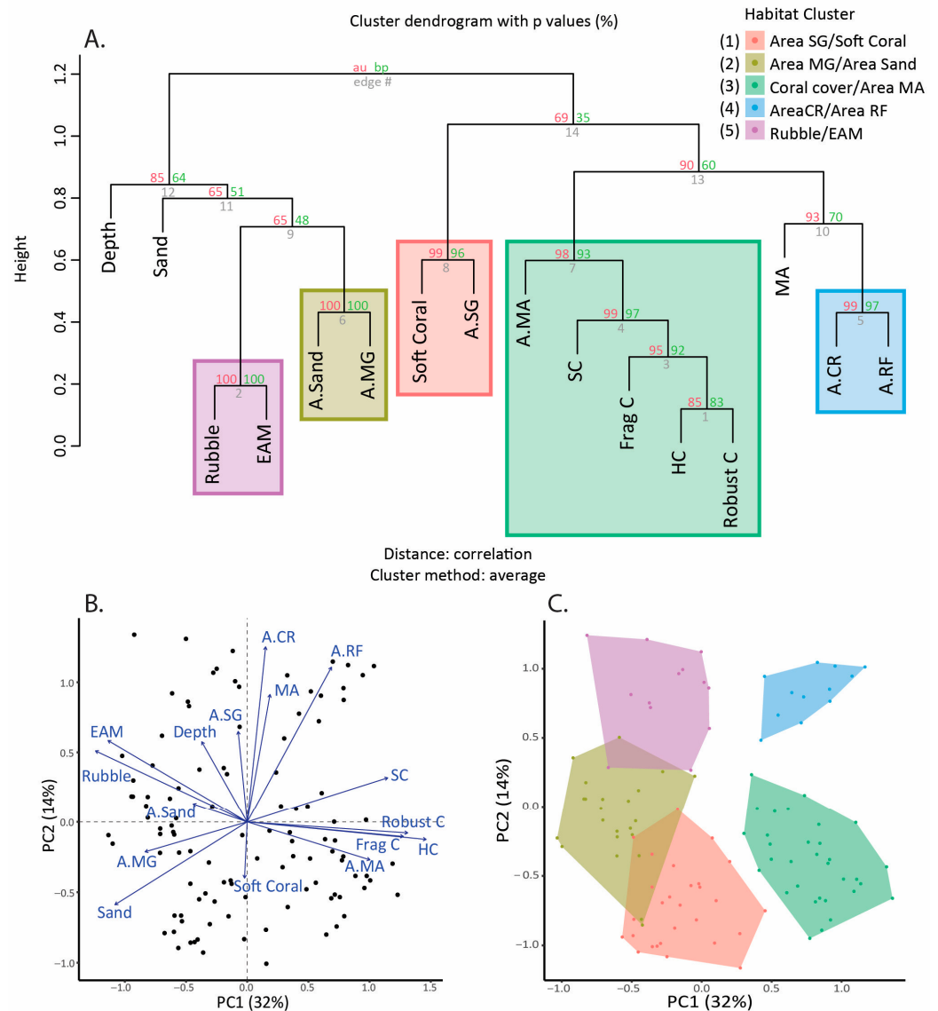
Figure 2. (A) Hierarchical cluster dendrogram of within reef benthic habitats and seascape measures of multiple habitats. At each branch, the left value (red) is the approximately unbiased (AU) p-value, and the right value (green) is the bootstrap probability (BP) p-value. The AU value is used to define habitat clusters, where branches with AU > 95% are significant. The numbers on the habitat cluster legend are the same as in Figure 1. A.MG = area of mangrove; A.MA = area of macroalgae; A.SG = area of seagrass; A.CR = area of coral reef; and A.RF = area of reef flat. SC = structural complexity. Frag C = fragile coral. HC = hard coral. Robust C = robust coral. MA = macroalgae. (B) Redundancy analysis (RDA) visualizing the variation in habitat variables along two principal component axes. Dots are individual transects, and vectors are plotted variables. (C) RDA grouped by habitat cluster identified in the hierarchical cluster analysis. Points are individual transects.
