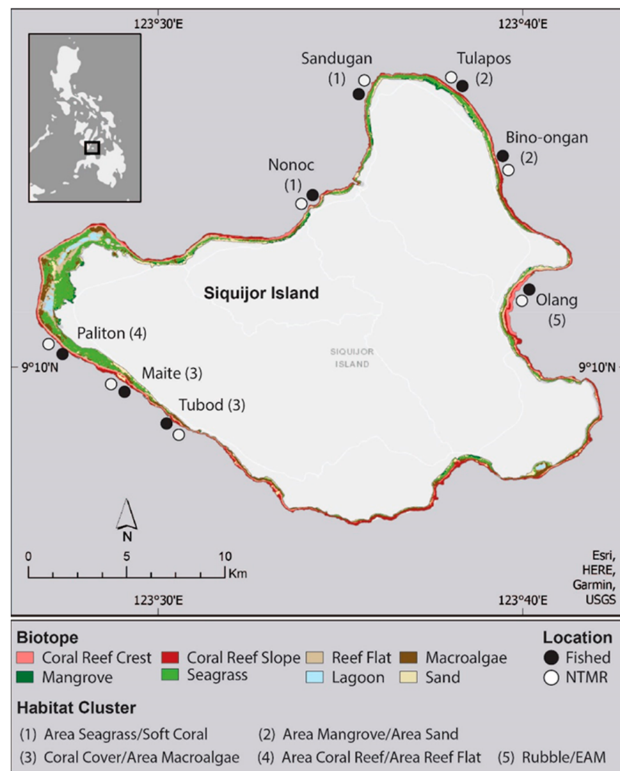
Figure 1. Map of Siquijor Island with classified submerged habitats. Black dots indicate the locations of fish and benthic habitat surveys conducted on coral reefs. For each location, a fished and no take marine reserve (NTMR) site was surveyed. Numbers represent habitat cluster identification based on k-means clustering analysis. Cluster describes the habitats within 500 m of survey sites, which characterizes the area identified by hierarchical cluster analysis.
