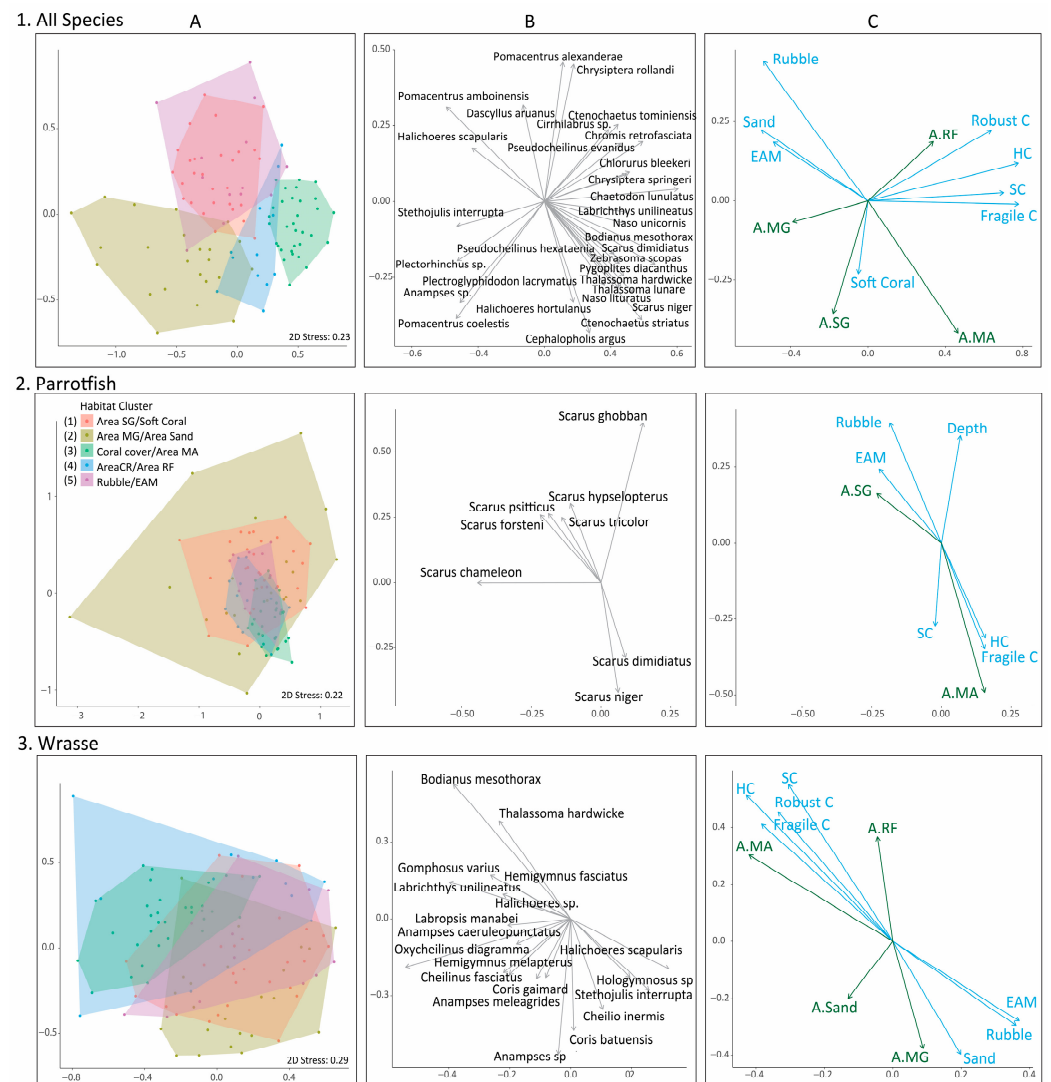
Figure 4. Fish assemblage results for all species observed (row 1), parrotfish (row 2), and wrasses (row 3). Column (A) displays the nonmetric multidimensional scaling (nMDS) analysis depicting similarities in fish assemblage structure among habitat clusters. Colored polygons are the different habitat clusters. MA = macroalgae; MG = mangrove; SG = seagrass; CR = coral reef; RF = reef flat. EAM = epilithic algal matrix. Column (B) displays the vectors of individual fish species with significant ( p < 0.05 ) correlations resulting from the envfit analysis. Column (C) displays habitat variables significantly ( p < 0.05 ) correlated to fish assemblage structure. Blue vectors and variables are within-habitat benthic variables describing coral reef habitat, and the green vectors are seascape-level variables describing the area of different habitat types. Fragile C = fragile coral; robust C = robust coral. HC = hard coral; SC = structural complexity.
