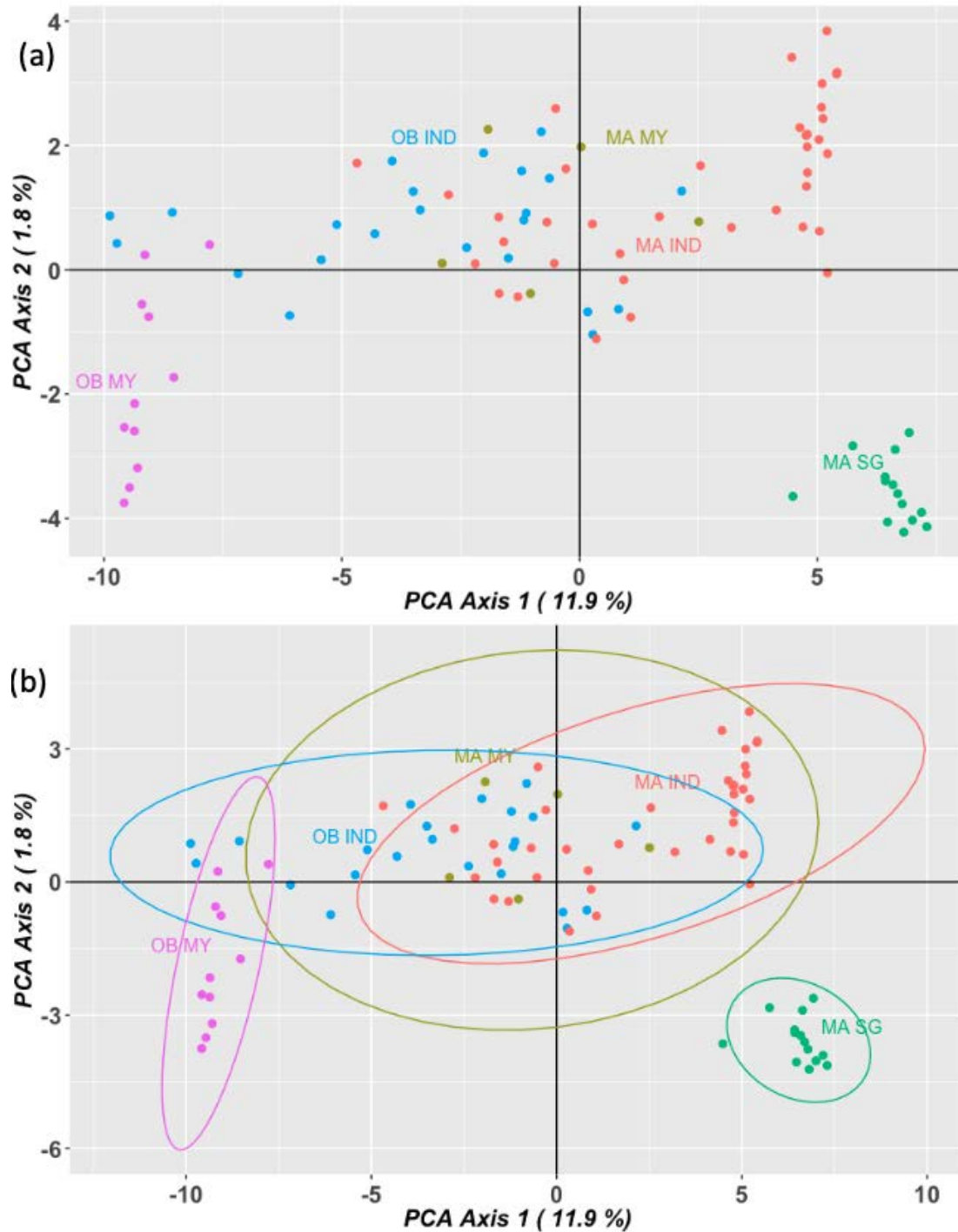
Fig 3.6. Principal Component Analysis (PCA) plot of nuclear DNA results for 92 bluespotted maskrays (a) without ellipses and (b) with ellipses. Individuals are labelled by species per the mitochondrial DNA result (OB = oriental bluespotted maskray, MA = mahogany maskray) and source population (IND = Indonesia, MY = Malaysia, SG = Singapore).
