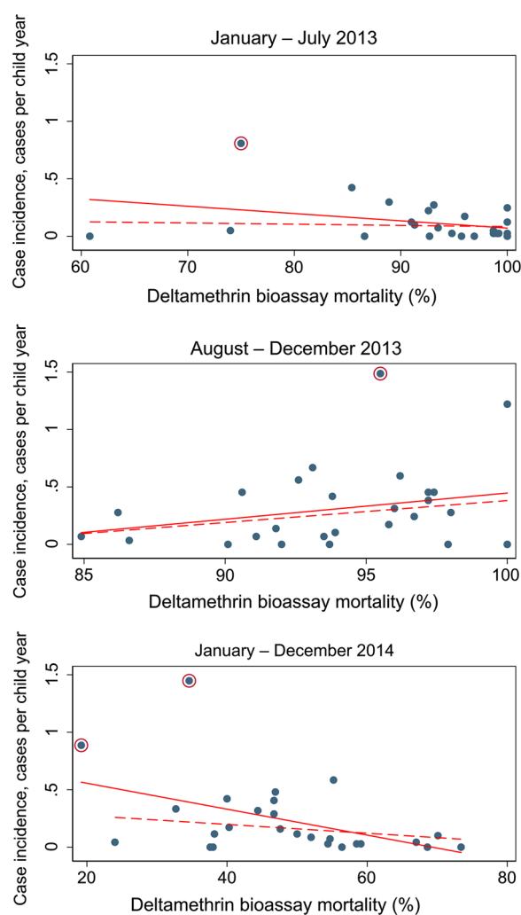
Fig. 4 Cluster level malaria mosquito mortality on exposure to deltamethrin versus rate of clinical malaria from a passively followed cohort of children under 5 years of age from January to July 2013 (top), August to December 2013 (middle), and January to December 2014 (bottom). Solid red lines represent lines of best fit; dashed red lines represent lines of best fit omitting outliers (these are the circled points defined as cluster level rate greater than 2 standard deviations above the mean cluster-level rate)
