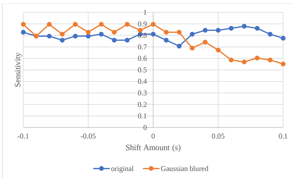
Figure 3.7 Sensitivity of GPATS.
