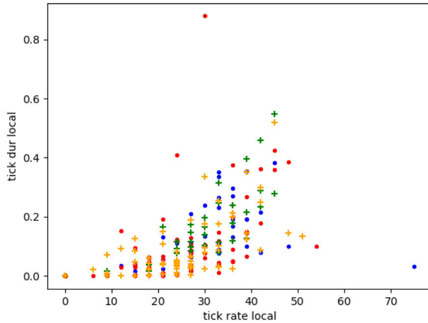
Figure 5.26 is the scatter plot between tick rate and tick duration.
