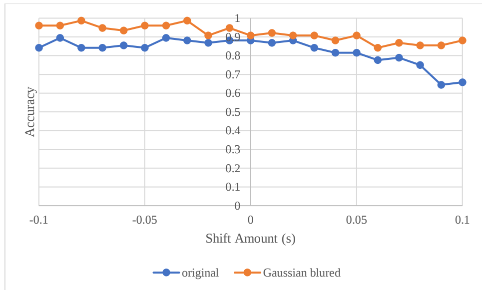
Figure 3.9 Accuracy of GMTS.
