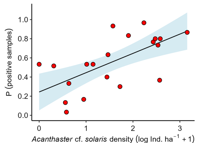
Fig. 5 Linear model fit (Table 3) of the proportion of positive eDNA samples versus recorded densities of A. cf. solaris using the SALAD method. The blue shaded area depicts the 95% confidence interval, the black line the model fit. Red dots are average observations per site and year
