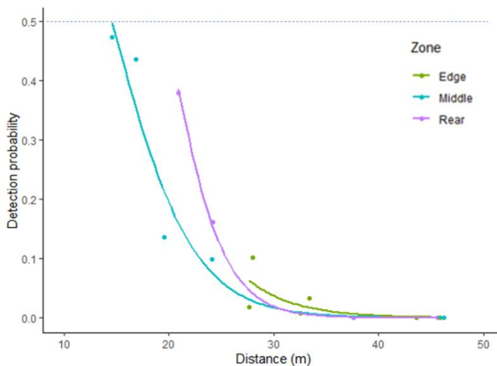
Fig. 4.6 Detection probability of the different zones for the inside mangrove test. Dotted line indicates 50% of detection probability. No detection was made by the flat receivers.
