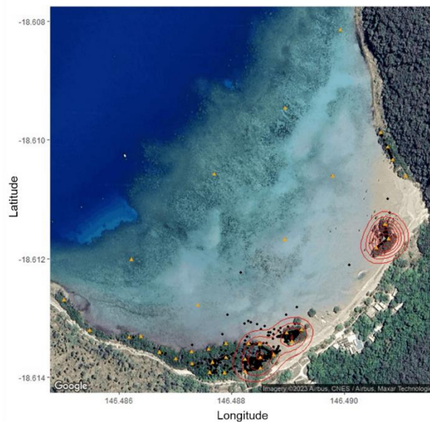
Fig. 5.7 Location of aggregation of juvenile mangrove whiprays. Black dots indicate the mean position of aggregation, red lines indicate the density of frequent aggregation locations and orange triangles indicate the receivers.
