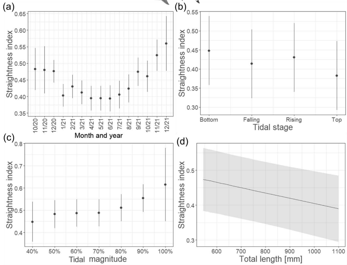
Fig. 5.8 Results of straightness analysis. (a) year-month, (b) tidal stage, (c) tidal magnitude and (d) body size.
