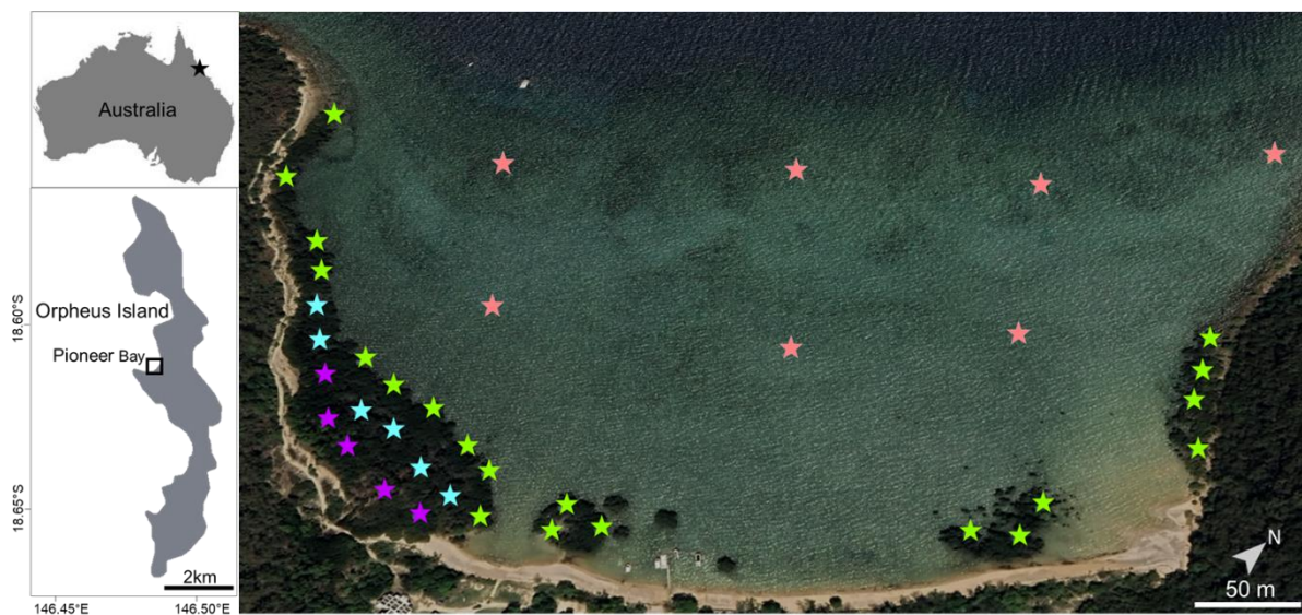
Fig. 5.1 Maps of study site and receiver deployment. Star indicates receiver (different zones in different colours: pink = zone 1: reef flat, green = zone 2: mangrove edge, blue = zone 3: mangrove middle and purple = zone 4: mangrove rear).
