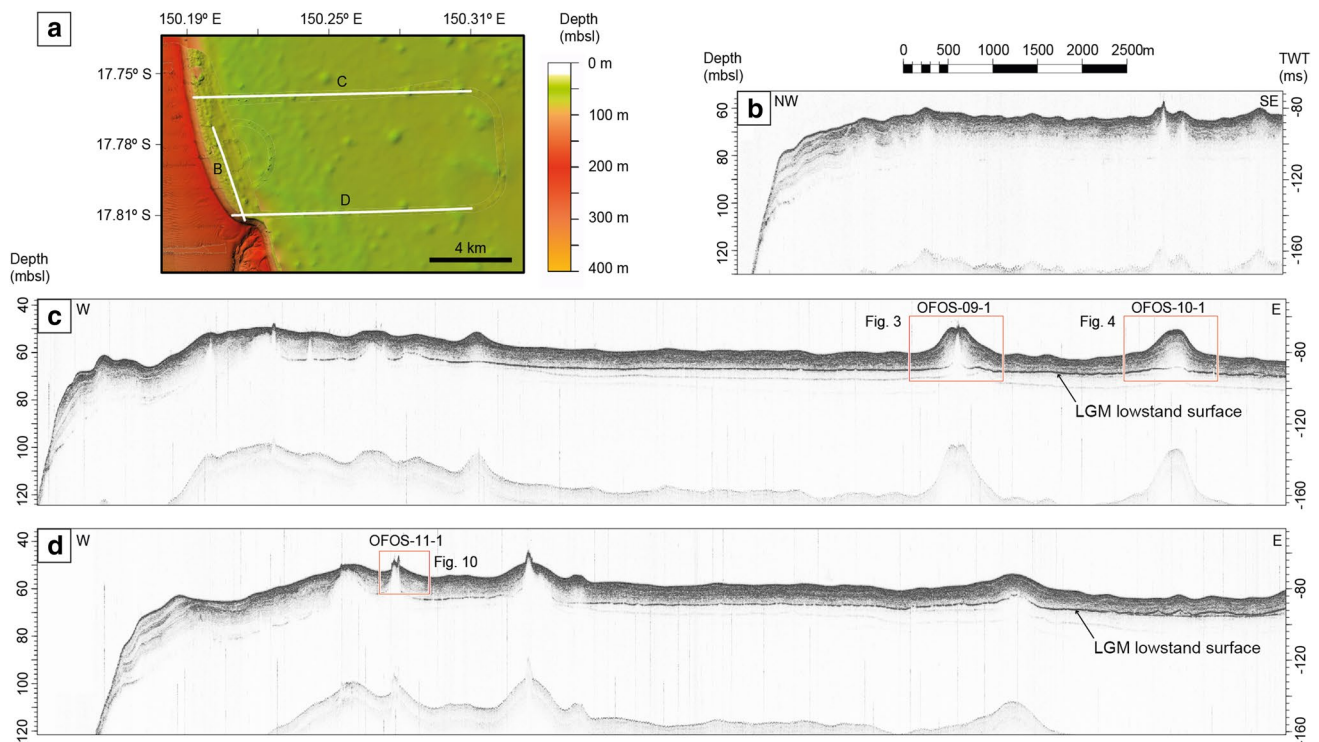
Fig. 2 Parasound profiles of the study area. A Bathymetry map with the locations of the Parasound lines at southwestern Tregrosse Bank. B–D Parasound profiles with the positions of the studied Halimeda mounds. LGM, last glacial maximum
