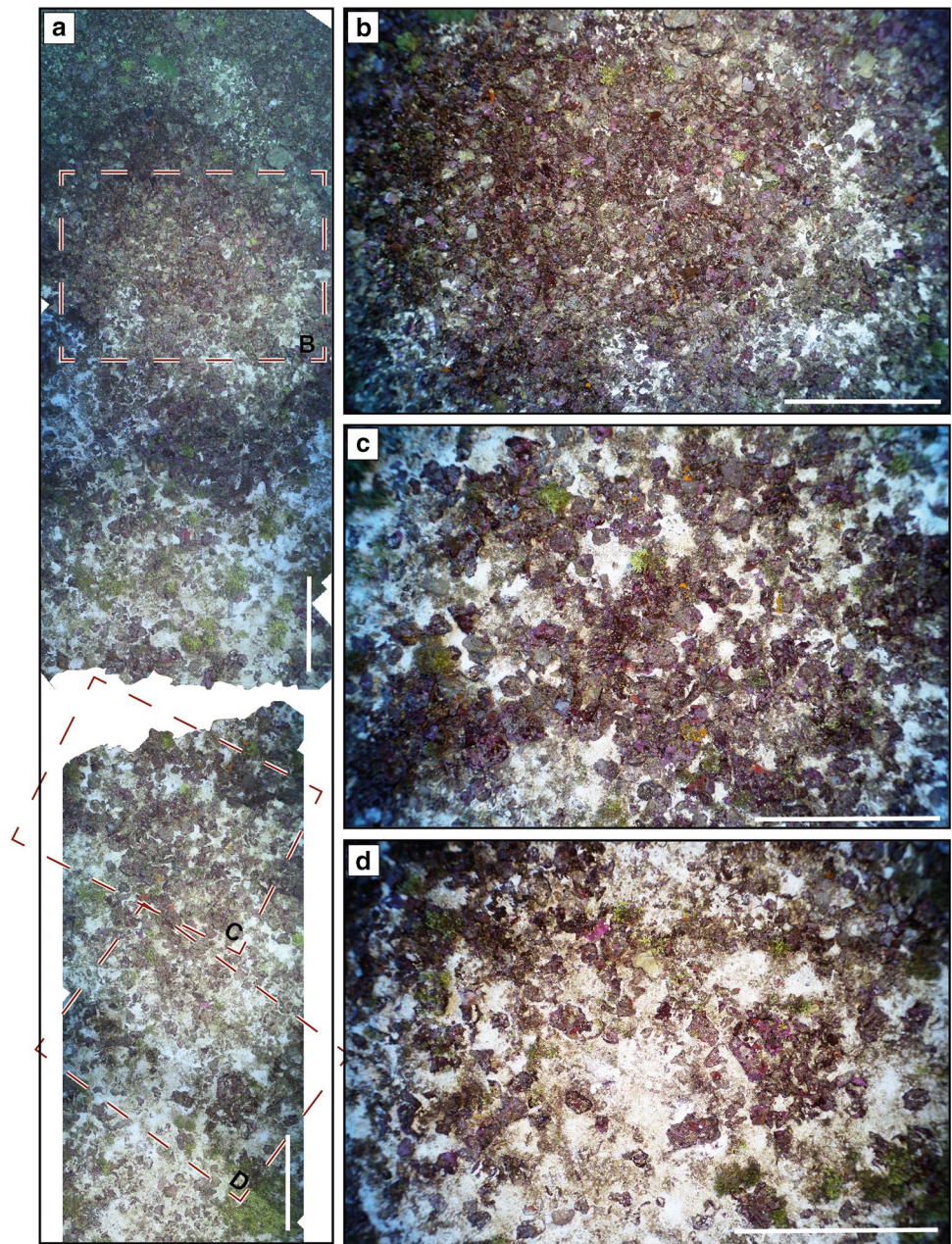
Fig. 8 Halimeda rudstone with coralgal debris at depths between 51 and 50 (OFOS station 09–1, Fig. 4). A Transect across the coralgal debris facies belt. Scale bar 1 m. Top of the bioherm is at the top of the picture. Dashed areas show the relative abundance of coralgal debris from B pavement of coralgal debris to C abundant, and D common coralgal debris on white Halimeda rudstone
