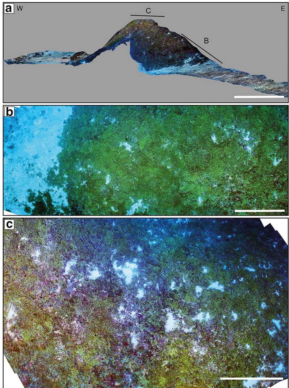
Fig. 10 Halimeda bioherm (OFOS station 11–1). A Photogrammetric model of the bioherm covered by living Halimeda plants. Scale bar 5 m. B Panorama of the toe of the bioherm with the transition from living Halimeda plants, green, to Halimeda rud- stone, white- coloured platform sediment. C Panorama view of the top of the bioherm. Scale bar 1 m
