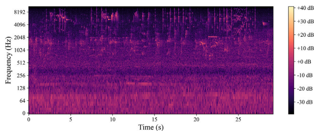
(a) Spectrogram of the audio signal, obtained through a Short-Time Fourier Transform (STFT).
