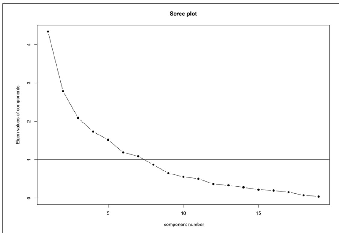
Fig. 2. Scree plot for the PCA in the V-CSDD study.
