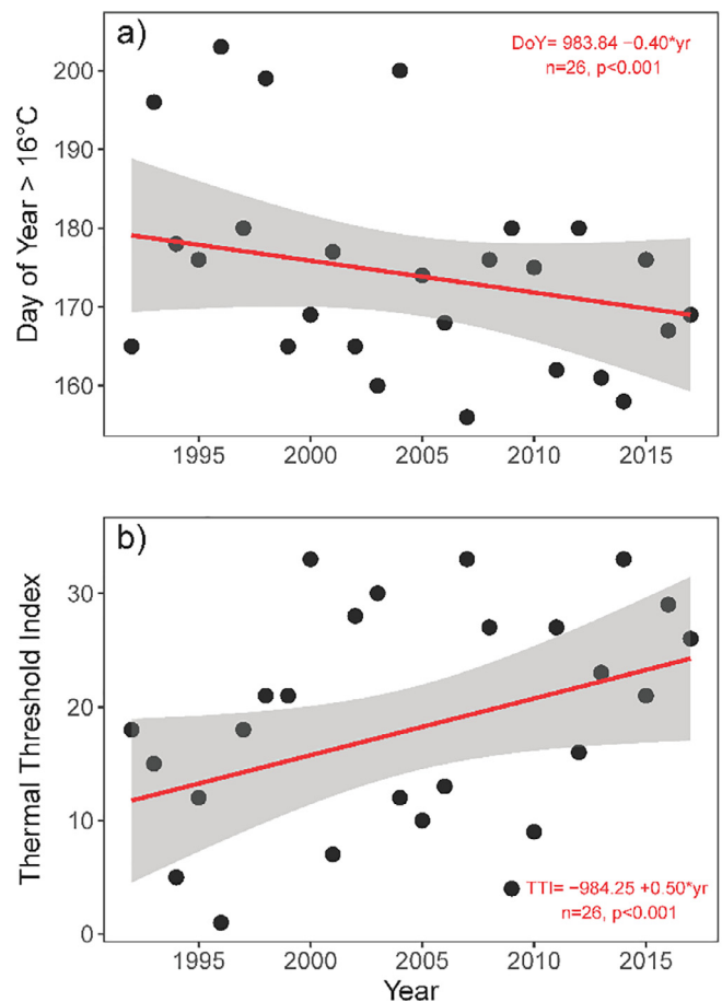
Fig. 3. Sea surface temperature in the Greifswald Bay in the 1992–2017 period. a) Day of the year (DoY) at which temperatures > 16 \text{ °C} were first reached for 8 consecutive days. Theil-Sen regression lines ( \pm 95\% CI) and equations are included in the graphs. Abbreviations: thermal threshold index, TTI (number of days > 16 \text{ °C} between March and June).
