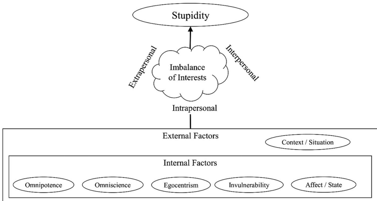
Figure 1. Imbalanced theory of stupidity.
