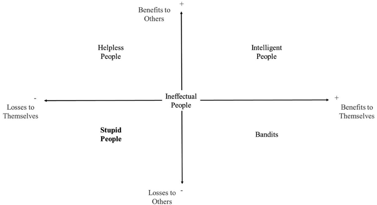
Figure 2. Cipolla’s theory of stupidity.
