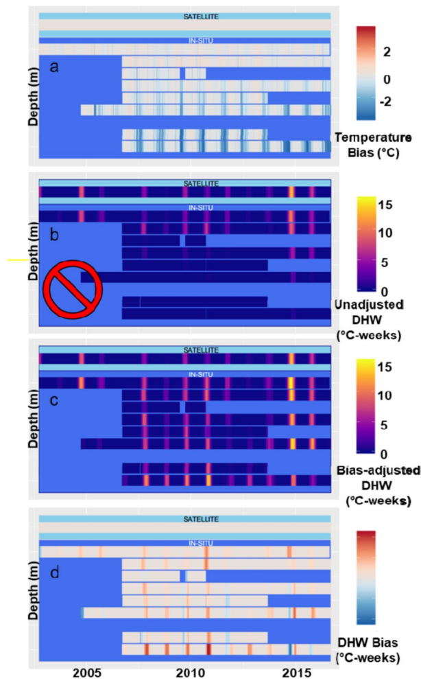
Figure 4. An example results of the new method of using bias-adjusted MMM to estimate DHW at depth of 38 m at Pearl & Hermes Atoll site between 2002 and 2016 (depths binned every 5 m, n = 30 ). (a) In situ (STR) temperature bias relative to satellite (SST) data (red = STR warmer, blue = STR cooler). (b) Subsurface DHW at depth using unadjusted MMM threshold (inappropriate in situ DHW calculation identified with red prohibition sign). (c) Subsurface DHW using bias-adjusted MMM threshold. (d) Difference between surface and bias-adjusted subsurface DHW (red indicates surface DHW is greater and blue indicates surface DHW lower than subsurface DHW).
