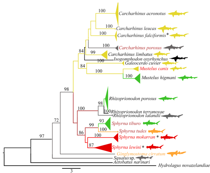
Figure 1. Neighbor-Joining tree for the NADH2 sequences of sharks from Brazil's North Coast. Sequences of Isogomphodon oxyrinchus , R. terranovae , Aetobatus narinari , and Hydrolagus novaezelandiae were obtained from NCBI – black branches. Bootstrap values below 70 are not shown. Branch colors follow IUCN extinction threat categories in Table 1 (dark red = CR, red = EN, orange = VU, yellow = NT, green = LC, gray = DD). Species with colored names are listed in Ordinance 445/2014. Asterisks correspond to species listed in CITES Appendix II.
