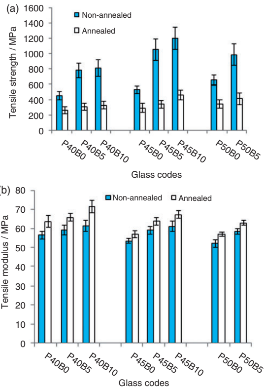
Figure 2. Tensile strength (a) and modulus (b) of annealed and non-annealed fibres in the glass system P_{40}Ca_{16}Mg_{24}Na_{(20-X)}B_x , P_{45}Ca_{16}Mg_{24}Na_{(15-X)}B_x and P_{50}Ca_{16}Mg_{24}Na_{(10-X)}B_x (where x = 0, 5 and 10 mol%). Error bars represent the standard deviation where n = 20 .
