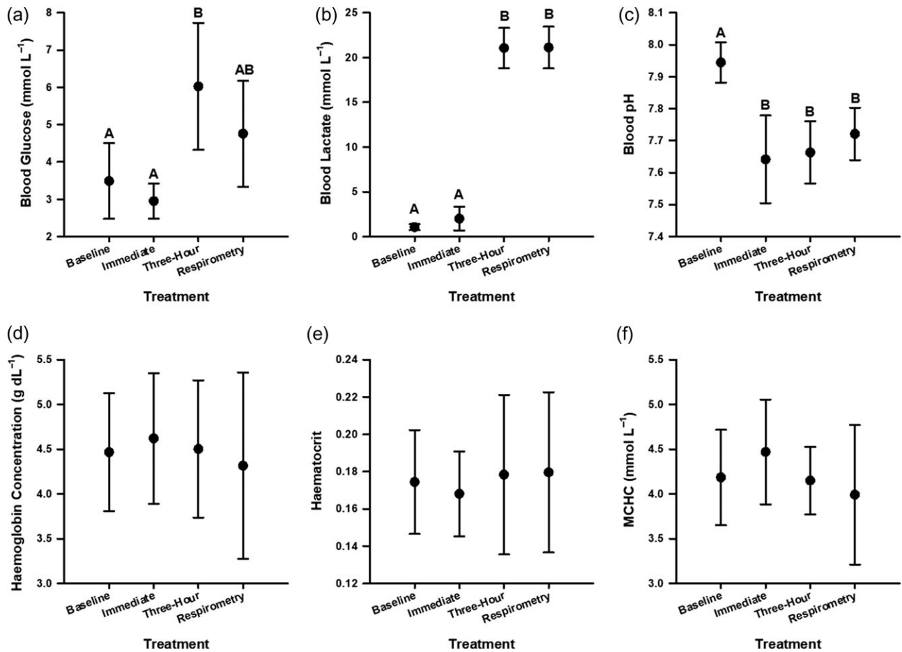
Figure 1: Indicators of the stress response in juvenile blacktip reef sharks ( Carcharhinus melanopterus ) following an exhaustive challenge in situ . Baseline values were taken from quiescent, fasted sharks (“baseline”). Other sharks were phlebotomized immediately following exhaustive gill-net capture (“immediate”), after three hours in a recovery bag (“three-hour”) or after 3 h in a field respirometry chamber (“respirometry”). Differing letters denote statistically significant differences. Abbreviation: mean cell haemoglobin concentration (MCHC).
