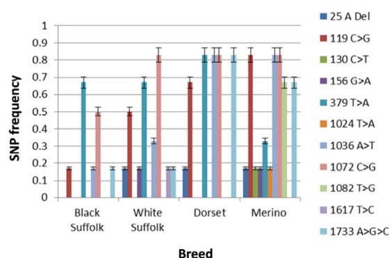
Figure 1: SNP frequencies in exon 1 and intron 1 by breed of sheep.
