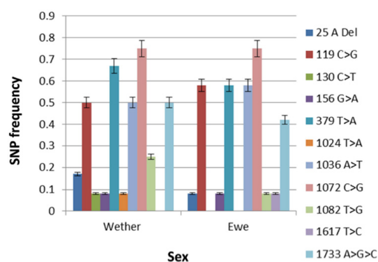
Figure 2: SNP frequencies in exon 1 and intron 1 in 17 wethers and ewes.
