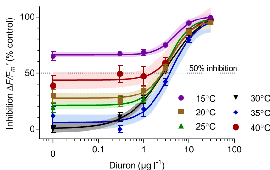
Figure 2. Concentration-response curves ( \Delta F/F_m' ) for diuron with H. ovalis at six temperatures. \Delta F/F_m' inhibition relative to 30^\circ\text{C} solvent control. All \Delta F/F_m' measurements were conducted under 100 \mu\text{mol photons m}^{-2}\text{s}^{-1} irradiance. Mean \pm SE of nine replicate leaf samples. Shaded areas represent the 95% confidence boundaries of each 4 parameter sigmoidal model.
