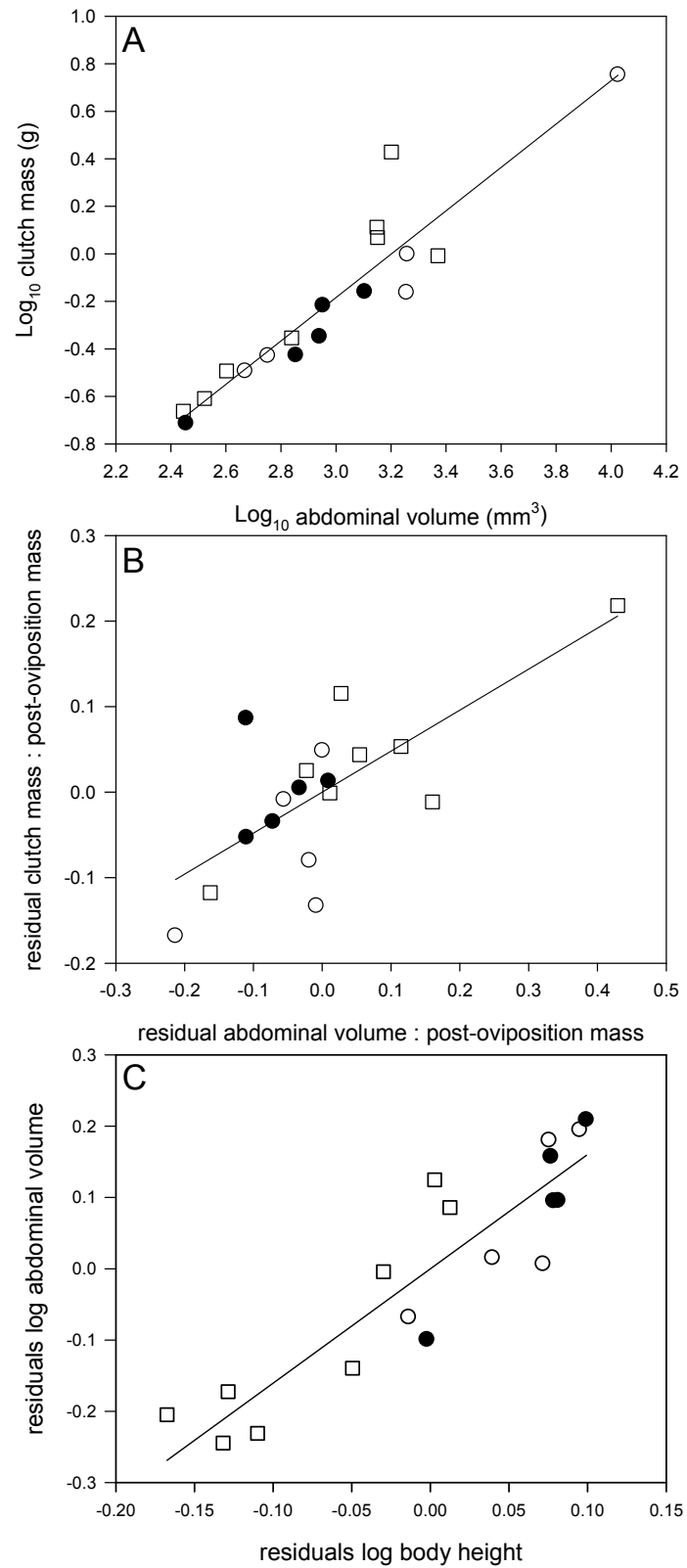
Figure 7.1. The relationship between A. abdominal volume and clutch mass B. residual abdominal volume and RCM and C. residual body height and abdominal volume of 18 species of scincid lizards. Refer to Chapter 6 for symbol legend.
