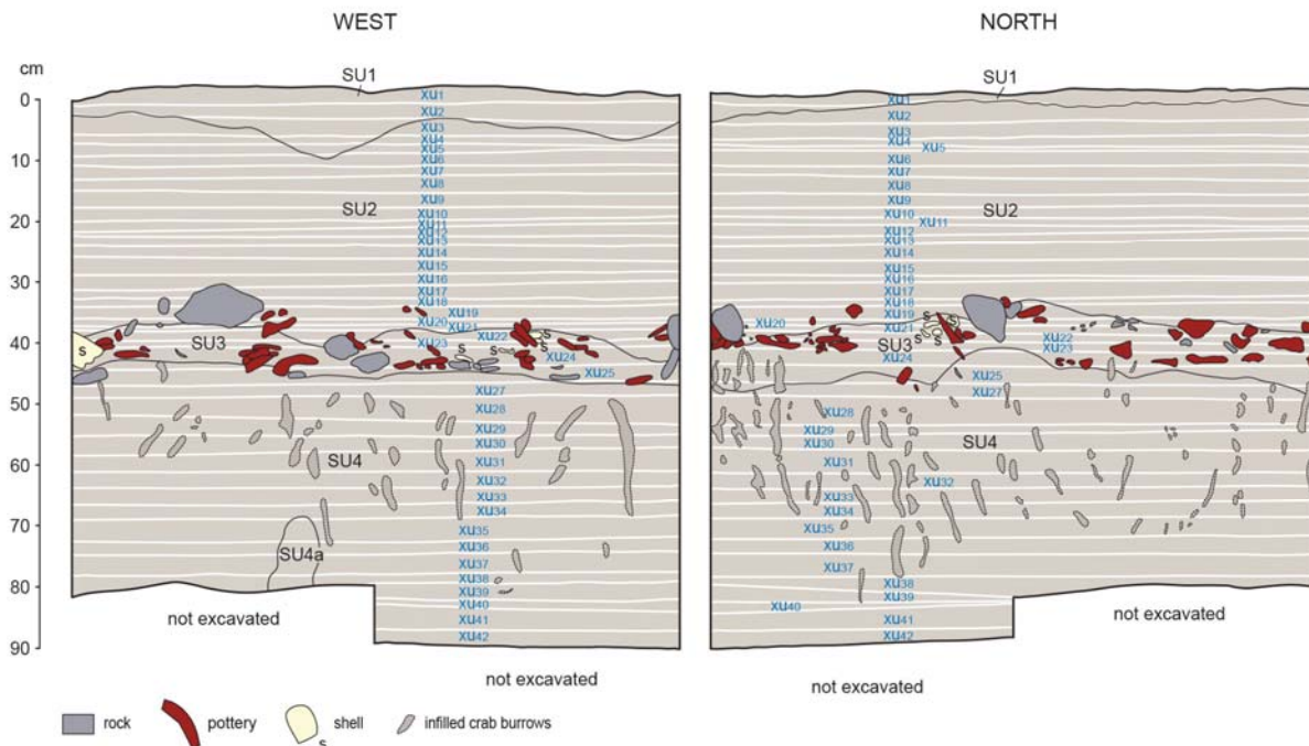
Figure 6. Ruisasi 1, west and north section drawings showing location of back-plotted XUs (XU26 does not reach as far as the west and north sections of the pit, i.e., that XU is not represented on Figure 6).
