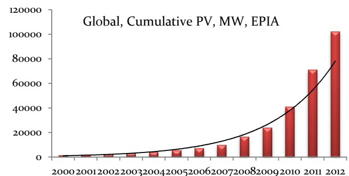
Figure 1 Cumulative PV Capacity MW
