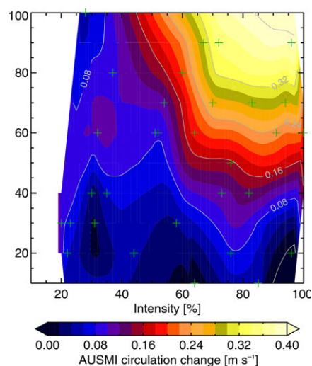
Fig. 13 Simulated differences between the fire scenario and the reference simulation of the response of the Australian Monsoon Index (AUSMI) [m s -1 ] to variation in fire intensity and burned area. AUSMI is obtained by averaging the daily mean 850 hPa zonal wind speed from the equator to 10°S and from 120°E to 150°E, the zone of monsoonal reversal of the flow in and out of Australia. The crosses indicate the population of the simulation space consisting only experiments with a timing of the fire-event later than the Julian day 250 (7 September). The contoured response metric is then Gaussian low pass filtered linear interpolations based on Delauney triangulations. Reprinted from Lynch et al. (2007, p. 4).
