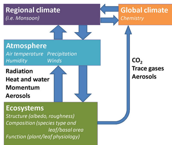
Fig. 2 The important linkages between the land surface and the earth system. Modification of ecosystems through fire will influence on ecosystem properties (structure, composition and function) and then through biophysical and biogeochemical feedbacks at multiple scales from local boundary layer to global climate. The important exchanges are listed using black bold-face text. Reprinted from Beringer et al. (2011a, p. 1467).
