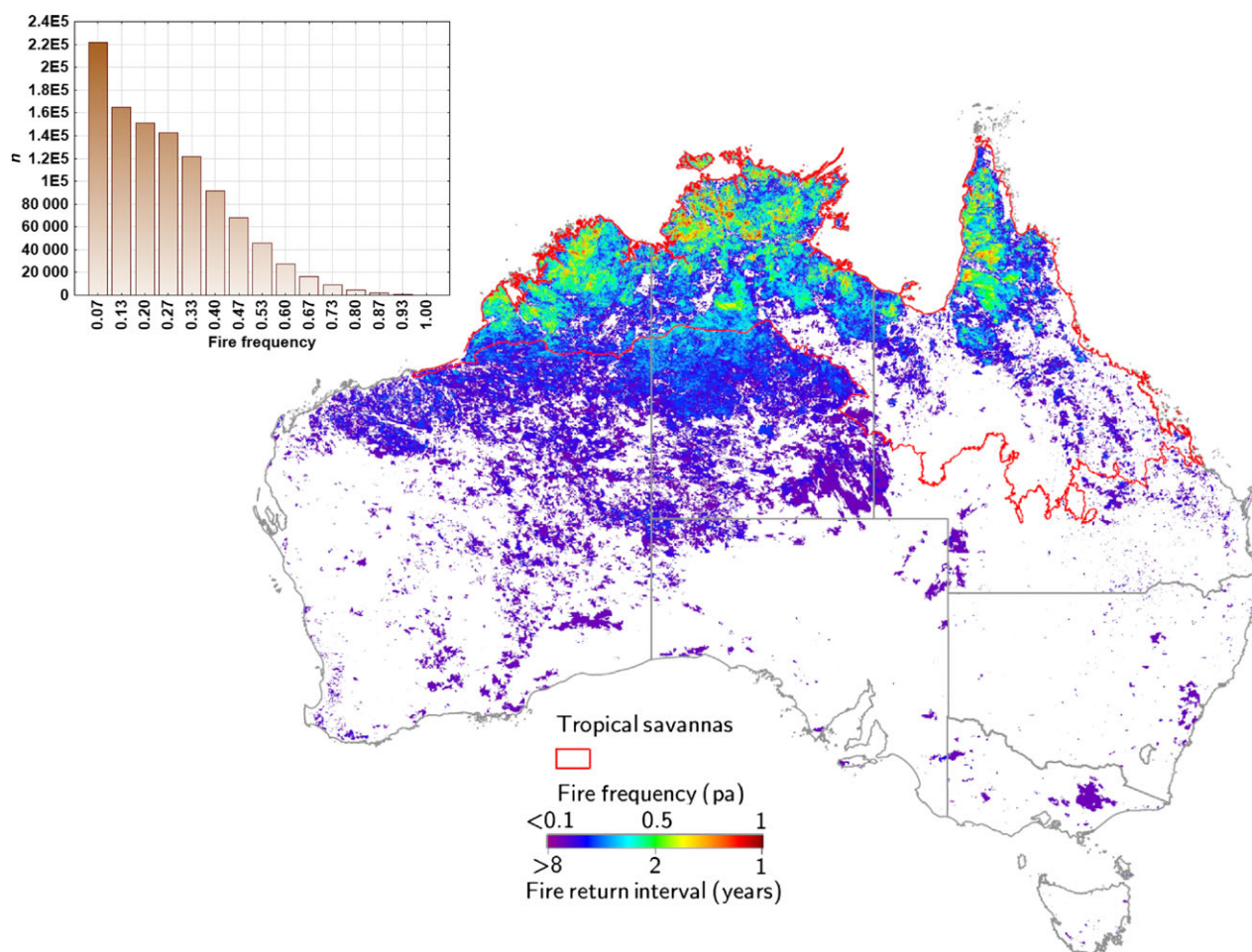
Fig. 3 Fire frequency of large fire events (generally >4 km 2 ) in Australia for the period 1997–2013 derived from AVHRR burnt area mapping. Frequencies range from less than 0.1 pa (dark blue) to 1 pa (dark red). Areas in white have not been marked as burnt during the mapping period. Tropical savannas are outlined in red (updated from Maier & Russell-Smith, 2012, p. 84). A histogram illustrates the spatial heterogeneity of fire frequency.
