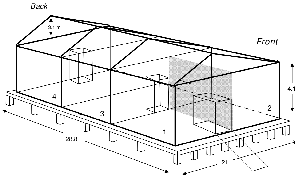
Figure 1 Schematic diagram of the IHI Semi-field system (SFS) for research on African Anopheles ecology and control.
