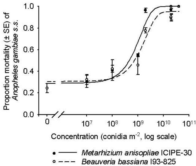
Figure 1 The percentage mortality of An. gambiae s.s. mosquitoes 3 - 6 d of age, 10 days post exposure to different concentrations of M. anisopliae ICIPÉ-30 and B. bassiana I93-825. Controls were not exposed to any fungus (0' concentration). Mosquitoes were exposed to the treatments for 6 h. The sigmoidal models were fitted to the data using probit regression.
