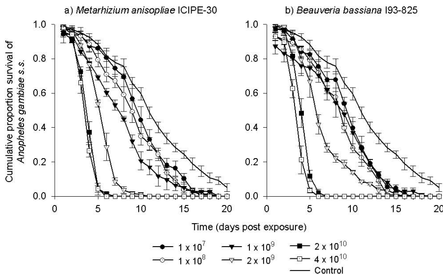
Figure 2 The survival of Anopheles gambiae s.s. females after 6 h exposure to different concentrations ( 1 \times 10^7 , 1 \times 10^8 , 1 \times 10^9 , 2 \times 10^9 , 2 \times 10^{10} and 4 \times 10^{10} conidia m^{-2} ) of a) Metarhizium anisopliae ICIPÉ-30 and b) Beauveria bassiana I93-825.
