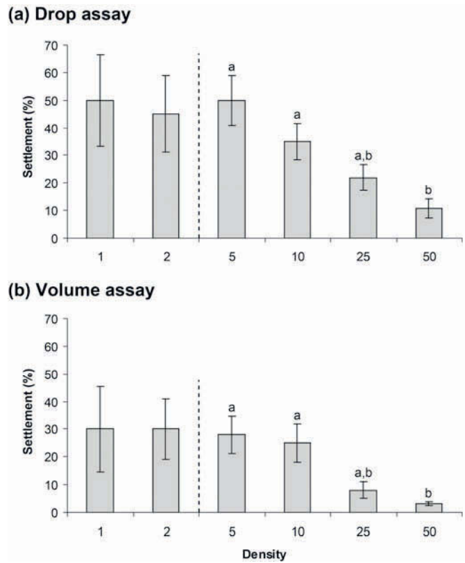
Figure 2.1: Settlement (%) of pediveligers of M. galloprovincialis after 48 h at different densities in (a) drop and (b) volume assays. Means \pm SE are shown ( n = 10 ). Superscript letters indicate significant differences (Tukey's HSD; \alpha = 0.05 ). Statistical analyses were only preformed for densities \geq 5 larvae per dish (to the right of the dotted line).
