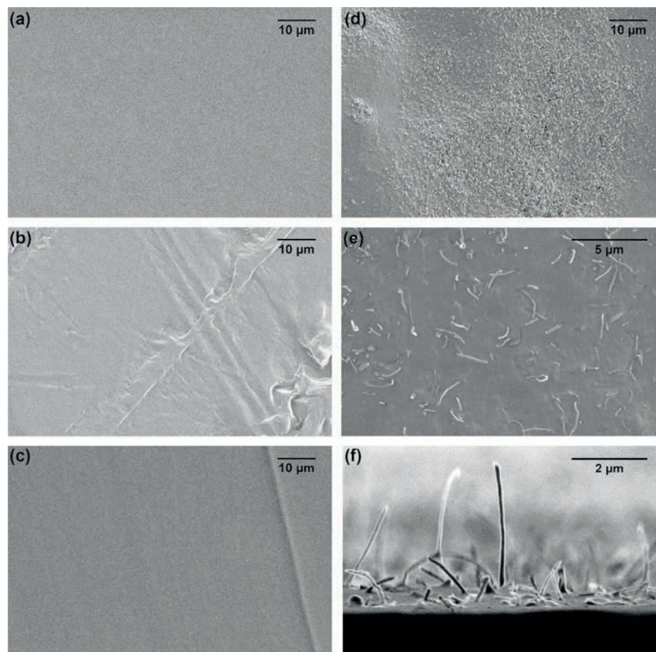
Figure 5.6: SEM images of (a,b) the surface and (c-f) cross-sections of (a,c) blank PDMS and (b,d-f) PDMS filled with 6 wt% CNTs. (d-f) Cross-sections of filled PDMS show CNTs protruding from the PDMS matrix where cut as illustrated in the (f) tilted view of a cross-section.
