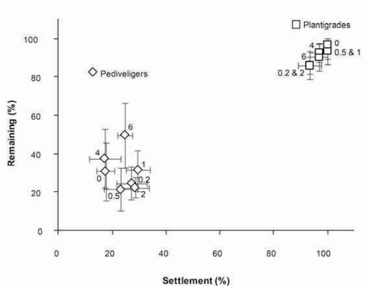
Figure 5.8: Correlation between initial settlement (%) and remaining (%) plantigrades and pediveligers of M. galloprovincialis on PDMS filled with CNTs (0.2, 0.5, 1, 2, 4, 6 wt%) after being exposed to a water flow of 4 knots for 2 min. The percentages of remaining pediveligers and plantigrades are based on the settlement on test surfaces. Means \pm SE are shown ( n = 6 ).
