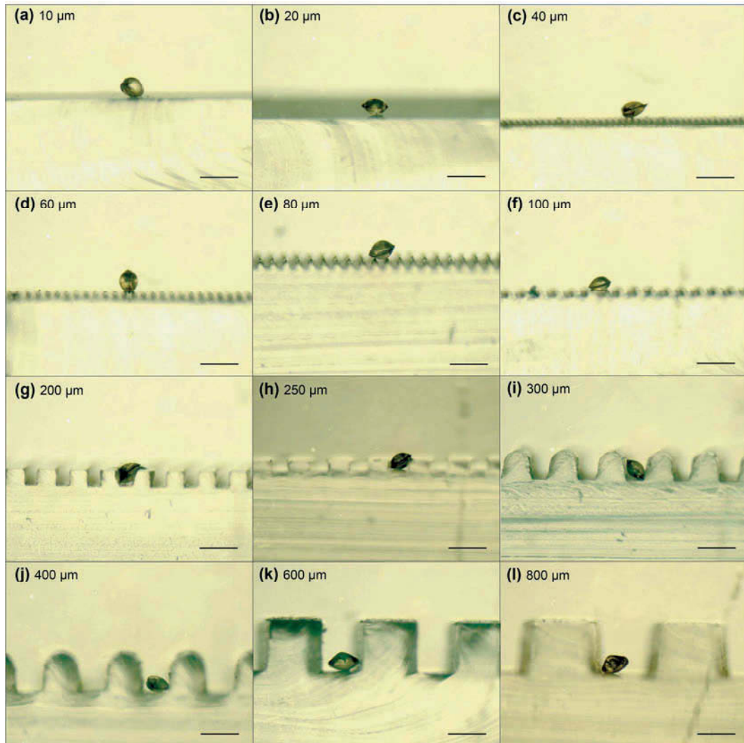
Figure 3.7: Cross-sections of the textured PDMS surfaces used in settlement assays with pediveligers of the mussel M. galloprovincialis on (a) 10 \mu\text{m} , (b) 20 \mu\text{m} , (c) 40 \mu\text{m} , (d) 60 \mu\text{m} , (e) 80 \mu\text{m} , (f) 100 \mu\text{m} , (g) 200 \mu\text{m} , (h) 250 \mu\text{m} , (i) 300 \mu\text{m} , (j) 400 \mu\text{m} , (k) 600 \mu\text{m} , and (l) 800 \mu\text{m} textured surfaces. Scale bars = 500 \mu\text{m} .
