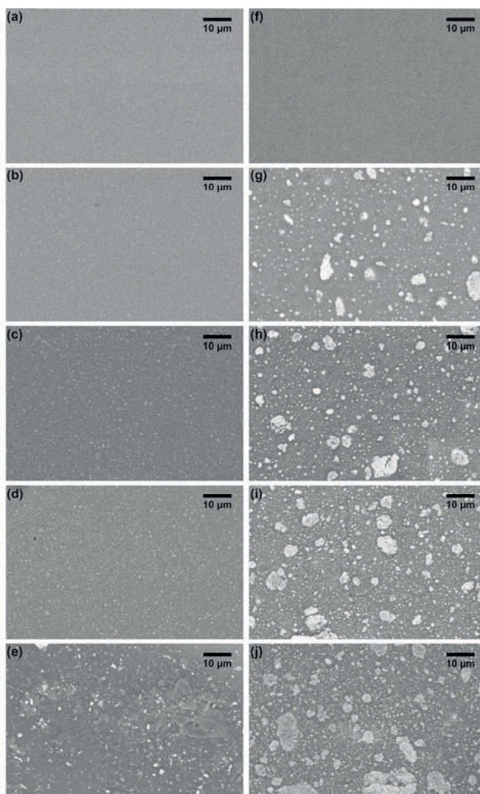
Figure 5.1: Backscattered SEM images of (a-e) the surface and (f-j) cross-sections through PDMS filled with various \text{TiO}_2 concentrations. (a,f) Blank PDMS control, (b,g) PDMS matrices filled with 3.75 wt% \text{TiO}_2 , (c,h) 7.5 wt% \text{TiO}_2 , (d,i) 11.25 \text{TiO}_2 , and (e,j) 15 wt% \text{TiO}_2 . Light coloured spots are \text{TiO}_2 particles.
