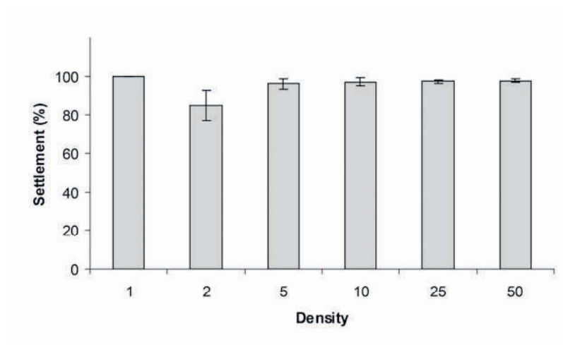
Figure 2.2: Settlement (%) of plantigrades of M. galloprovincialis after 6 h at different densities in volume assays. Means \pm SE are shown ( n = 10 ).
