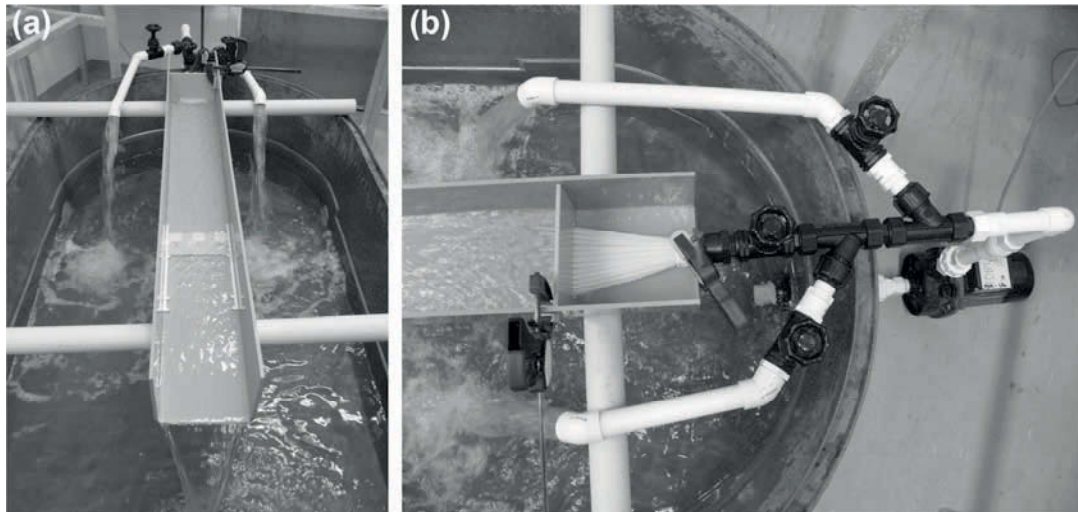
Figure 3.1: Flow chamber set up. (a) Front view of the raceway with a height of 130 mm, length of 1400 mm and a width of 150 mm. The samples were placed in a PVC frame, which was then placed in the raceway and secured using customised fittings. (b) The water is pumped into the raceway and dispersed through a PVC fitting filled with 23 small pipes orientated in the direction of the flow to ensure a homogeneous, laminar-like flow (Image courtesy of M.J. Vucko, JCU).
