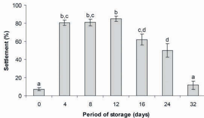
Figure 2.4: Settlement (%) of pediveligers of M. galloprovincialis stored at 4°C over 32 days. Settlement was determined after 48 h. Means \pm SE are shown ( n = 9 ). Superscript letters indicate significant differences (Tukey's HSD; \alpha = 0.05 ).
