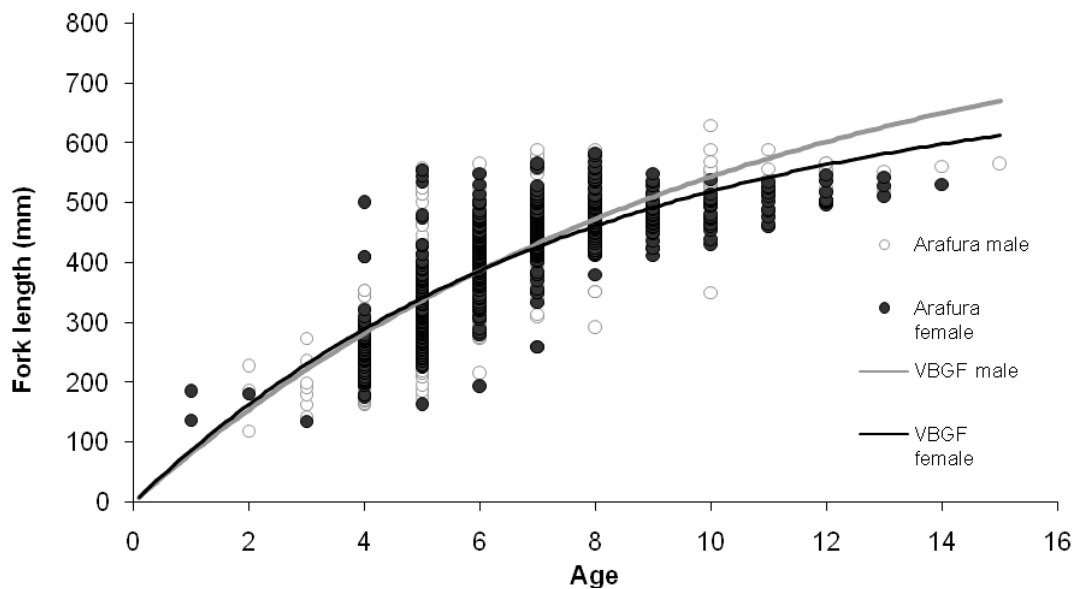
Figure 3.3.11b. Fork length at age and fitted VBGF curves for Pristipomoides multidens males and females for the Arafura Sea
