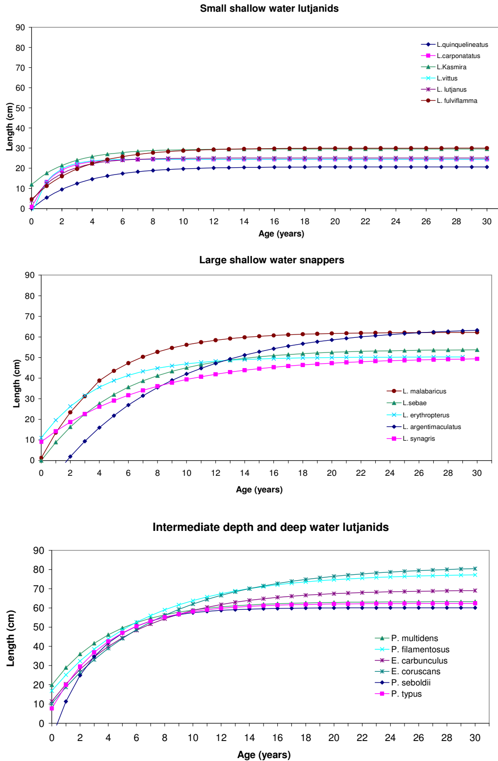
Figure 3.4.5. Comparison of generalised von Bertalanffy growth curves from the literature with respect to depth range. Growth curves have been constructed to age 30 years for the purposes of species comparison, but this does not indicate the maximum age of a species.
