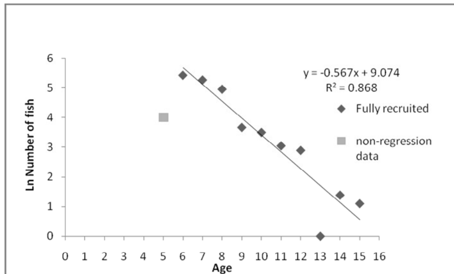
Figure 3.3.18. Catch curve obtained from fitted regression to log transformed number of Pristipomoides multidens in each age class from the Timor Sea. Only data from age classes which were fully recruited to the fishery were used for regression analysis
