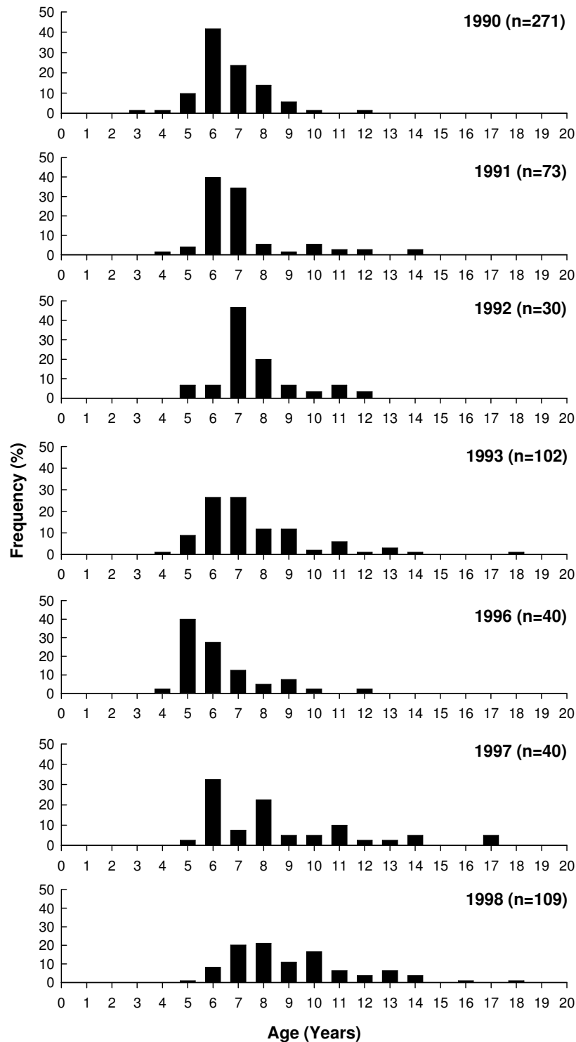
Figure 3.3.16. Age-frequency distribution of goldband snapper ( Pristipomoides multidens ) from the Timor Sea (1990-1998)
