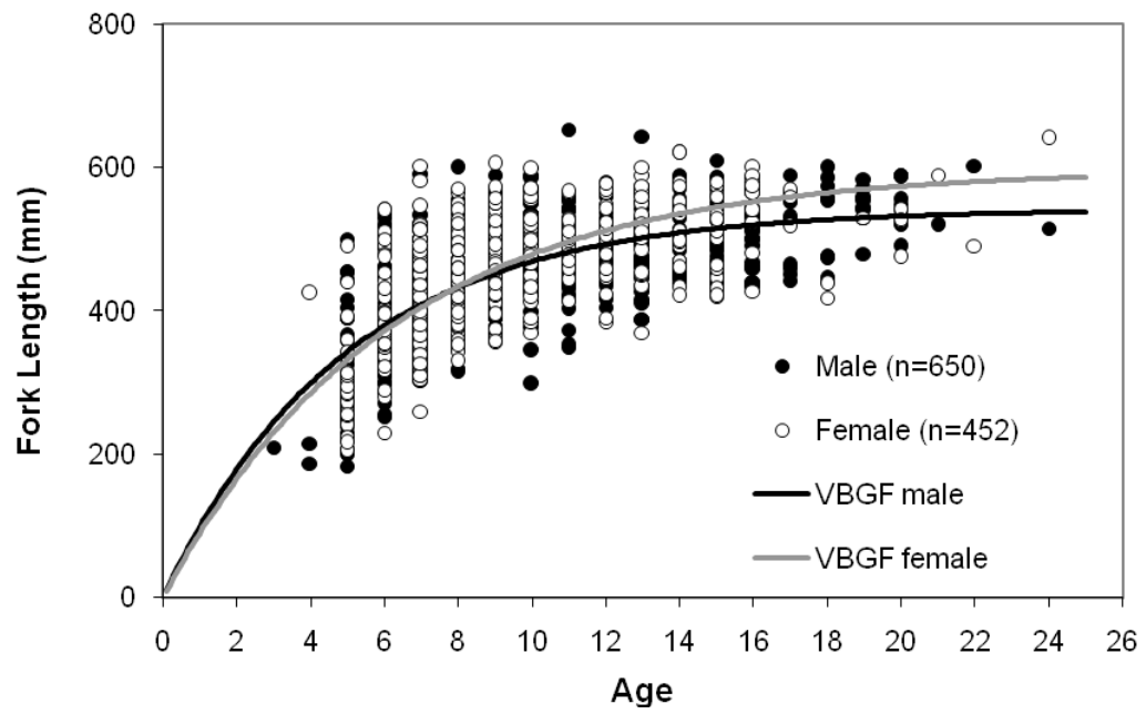
Figure 3.4.4. Fork length at age and fitted von Bertalanffy growth function for Pristipmoides typus
