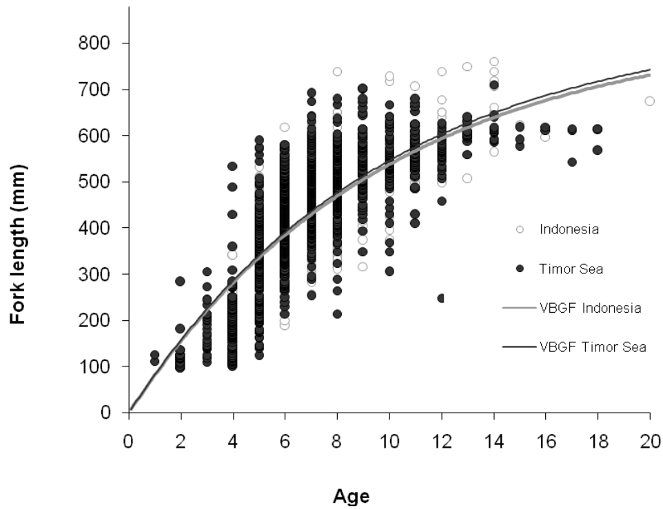
Figure 3.3.11d. Fork length at age and fitted VBGF curves for Pristipomoides multident (sexes combined) from Australian and Indonesian waters
