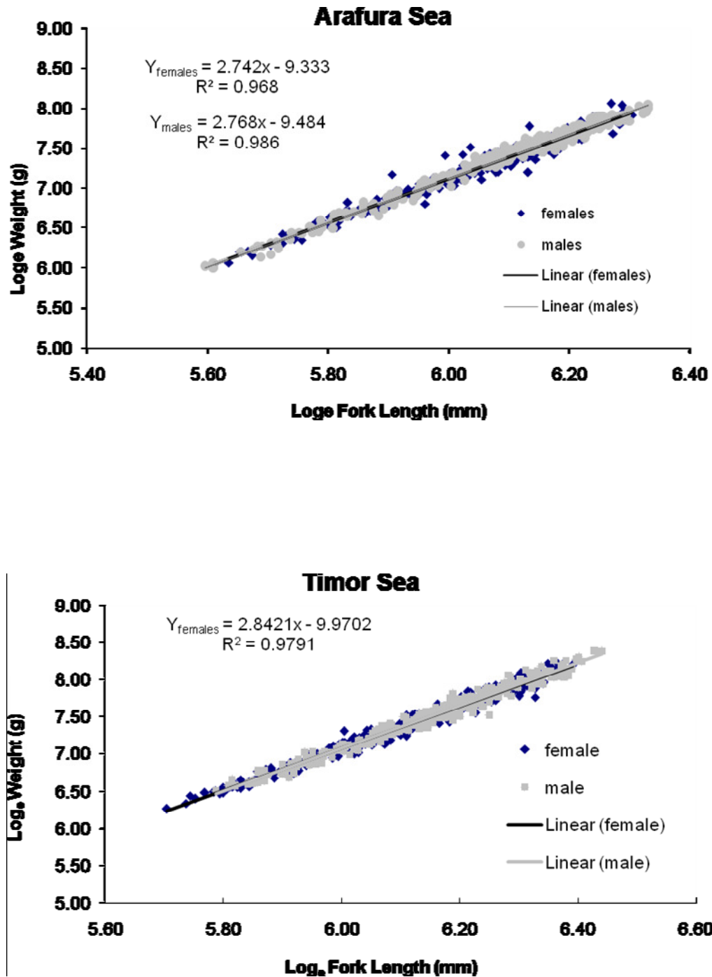
Figure 3.3.2. Log e transformed length-weight relationship for goldband snapper ( Pristipomoides multidentis ) from the Timor and Arafura Seas by sex
