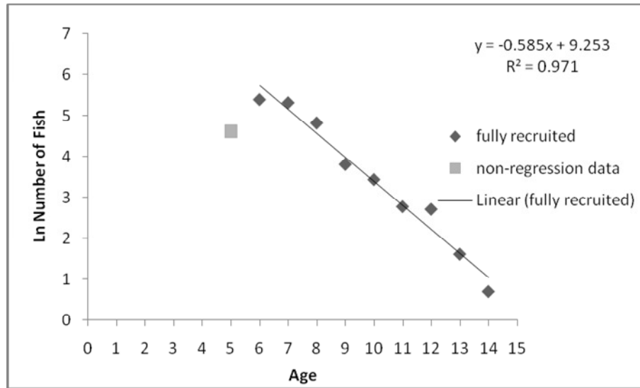
Figure 3.3.17. Catch curve obtained from fitted regression to log transformed number of Pristipomoides multidens in each age class from the Arafura Sea. Only data from age classes which were fully recruited to the fishery were used for regression analysis
