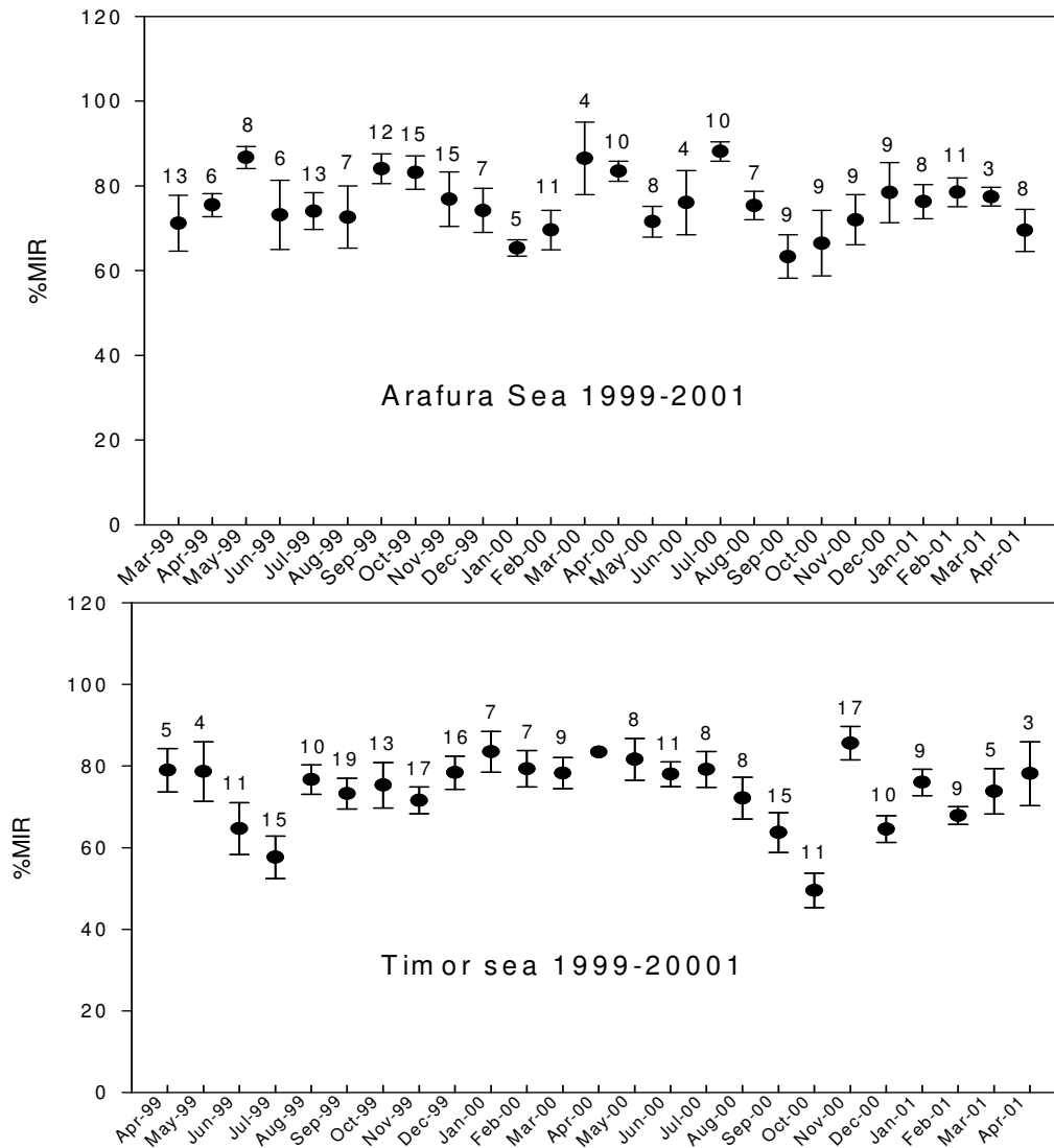
Figure 3.3.7. Mean monthly increment ratio (MIR) \pm standard error by location for Pristipomoides multidentis . Samples size is shown above each data point
