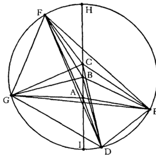
Figure 16: The Vicarious Hypothesis, taken from Kepler's own diagram in Chapter 16 (after Kepler, 1992: 252).
