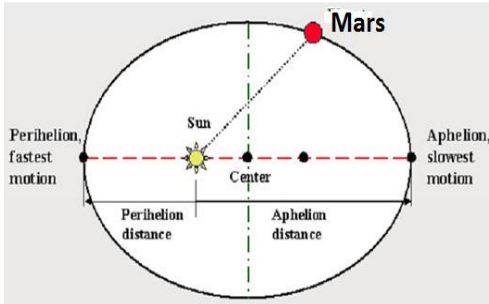
Figure 15: The orbit of Mars (adapted from Wikimedia).
