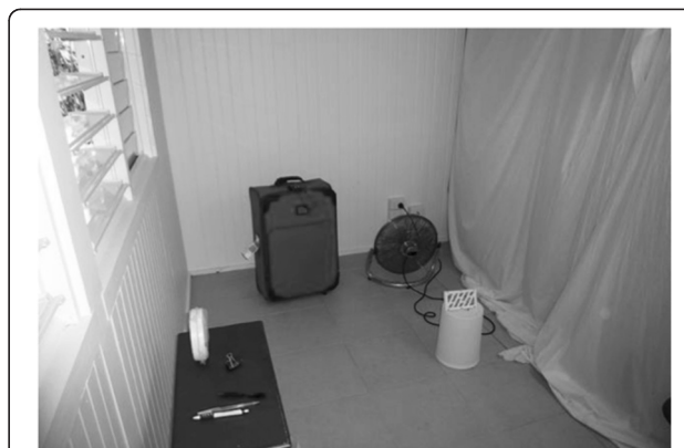
Figure 1 Experimental room 3. Room used in open room trials showing a suitcase, metofluthrin emanator (on bucket), open louvered window and Clark sentinel ring on table. The small table fan was turned on low and faced away from the emanator, generating wind speed of 0.2 m/s at the emanator located 1 m way.
