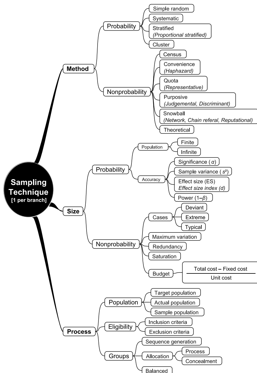
Figure 3.4 Sampling technique
