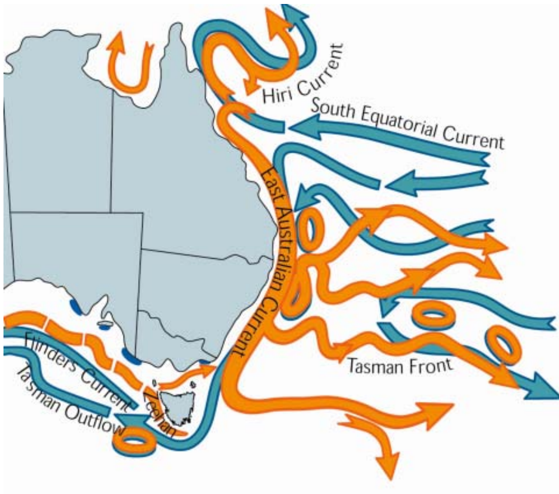
Figure 1.2: Ocean currents in the south-west Pacific and Coral Sea (from Ridgway and Hill 2009). Surface currents are shown in orange and subsurface currents in blue.
