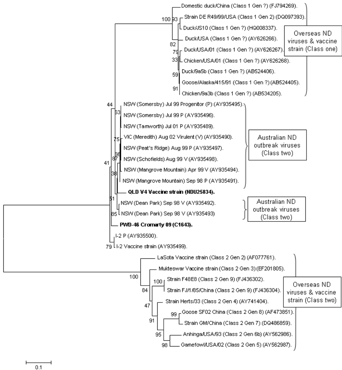
Figure 5.2 Bootstrap consensus trees with 5,000 replications for the Newcastle disease viral matrix gene (nucleotide positions between 237 and 908 base pairs)
