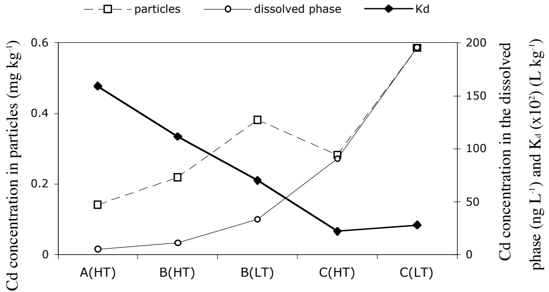
Figure 4.3: Mean temporal variation of K_d , Cd concentration in the dissolved phase and Cd concentration in the particles over the sampling sites: at site A during the high tide, A(HT), site B at high tide, B(HT) and at low tide, B(LT), and at site C at high tide, C(HT) and at low tide, C(LT).
