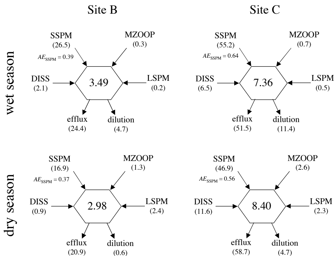
Figure 5.5: Budget models for site B and C in the wet season of 2004 and dry season of 2002. The Cd fluxes from the dissolved phase (DISS), SSPM, microzooplankton (MZOOP) and LSPM to Balanus amphitrite and the decrease in Cd concentration (efflux and dilution) are represented. Cadmium fluxes (in brackets) are in \mu\text{g kg}^{-1} \text{d}^{-1} , and Cd concentrations in barnacles (within hexagons) are in \text{mg kg}^{-1} .
