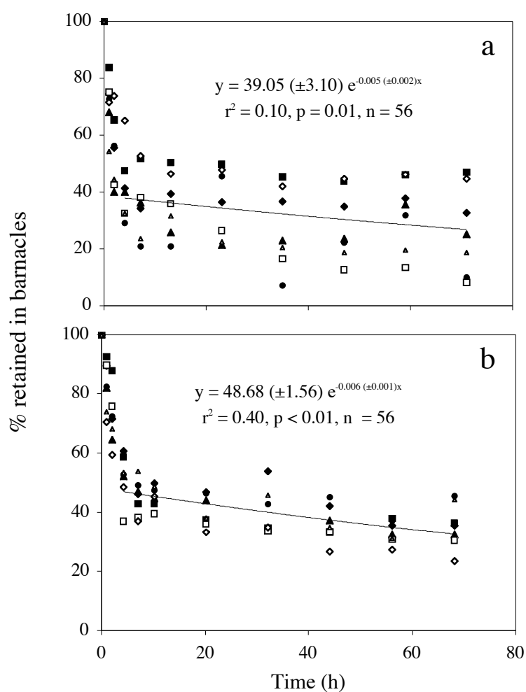
Figure 6.7: Retention of ^{109}\text{Cd} in 14 barnacles after seven of them been fed with SSPM poor in chl a (a) and the other seven been fed with SSPM rich in chl a (b). Numbers in brackets stand for the standard error of the parameter in the adjusted model. Different symbols stand for each of the seven barnacles fed with each batch of SSPM.
