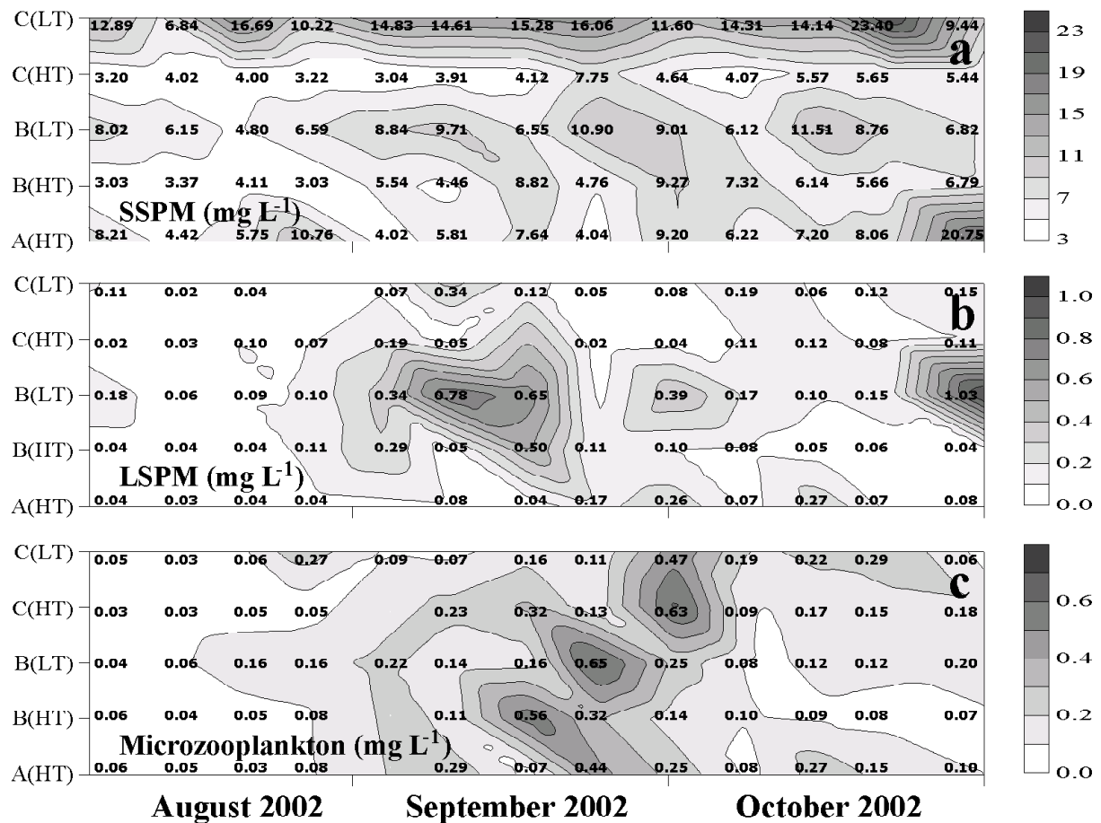
Figure 4.1: Mass concentration (mg L -1 ) of (a) SSPM (0.45–50 \mu m), (b) LSPM (50–200 \mu m) and (c) microzooplankton (50–200 \mu m), sampled from 6 August to 30 October 2002 in Ross Creek at site A during the high tide, A(HT), site B at high tide, B(HT) and at low tide, B(LT), and at site C at high tide, C(HT) and at low tide, C(LT).
