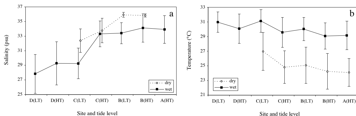
Figure 3.4: Mean water salinity (a) and temperature (b) measured at the low tide (LT) and at the high tide (HT) at sites A, B, C and D along Ross Creek in the dry season of 2002 and the wet season of 2004. Bars stand for \pm 1 SD.
