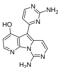
(6) Variolin B
