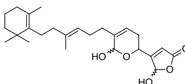
(14) Manoalide
