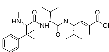
(10a) HTI 286
