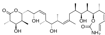
(8) Discodermolide
