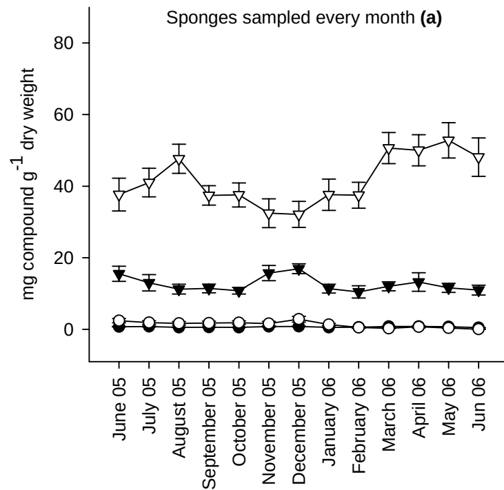
Figure 3.2a: Fine scale monthly production (mean concentration \pm SE)
