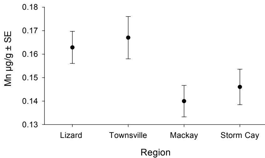
Figure 2.4 Mn µg/g concentrations (mean ± SE) in otoliths of 4-year-old P. leopardus collected in four regions on the GBR. Data were pooled across reefs and cohorts.
