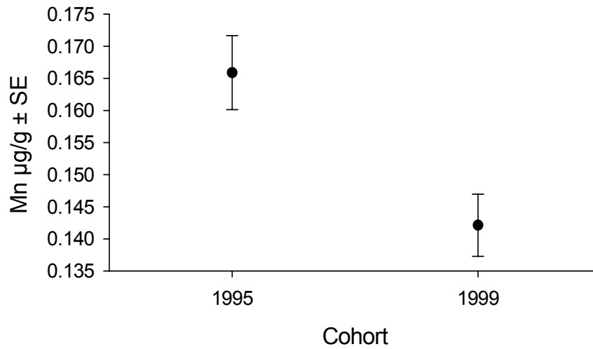
Figure 2.3 Mn µg/g concentrations (mean ± SE) in otoliths from two cohorts of 4-year-old P. leopardus , GBR. Data were pooled across reefs and regions.
