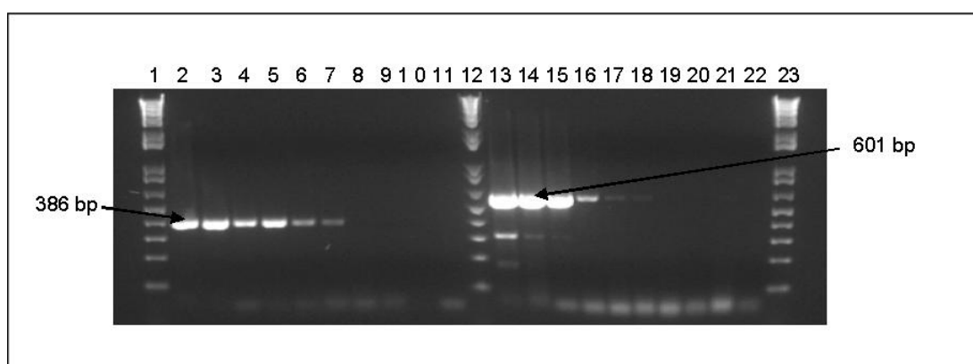
Figure 4.6 Electrophoresis of CAV PCR products
