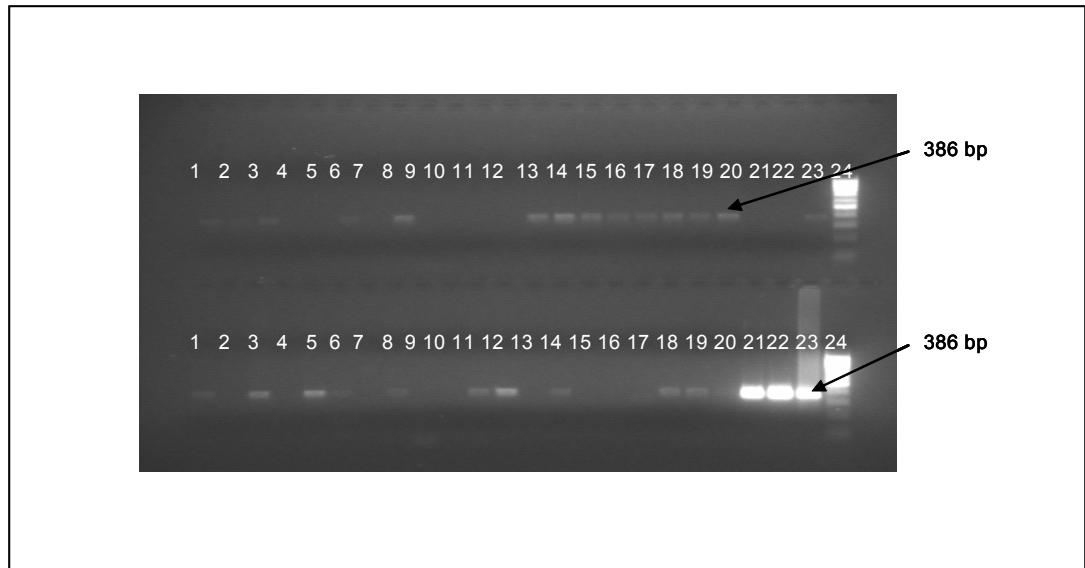
Figure 8.2 Electrophoresis of first round PCR. Template: 2 \mu l sample DNA, Primers CAV Cux - O3F and O3R
