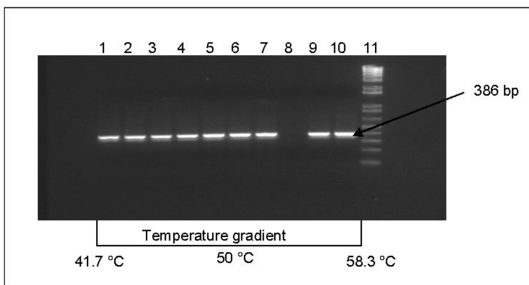
Figure 4.2 Agarose gel electrophoresis of CAV PCR products Annealing temperature gradient programmed PCR assay with different temperature in each, well Primer: CAV O3F and O3R, template: CAV DNA of strain 3711, Lane 1-10: 2.5 mM Mg +2 concentrations, Lane 11: Marker, 100 bp DNA ladder plus, In the lane eight, there was no template due to an error in template loading
