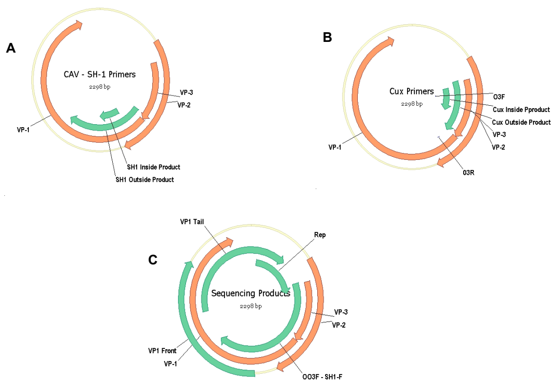
Figure 3 CAV circular genome with VP, VP2, VP3 protein and non-coding region A Diagnostic nested primer, CAV-SH-1 location in the genome. B Next diagnostic nested primer, Cux location. C Primers used for sequencing and their location in the genome.
