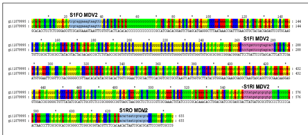
Figure 2 Primer sequence and location in the genome of published sequences of Gallid herpesvirus type 3 nuclear DNA binding protein gene at an inverted repeat region.
