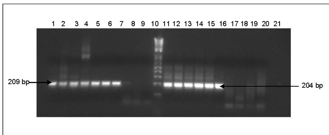
Figure 4.7 Electrophoresis of nested PCR products
