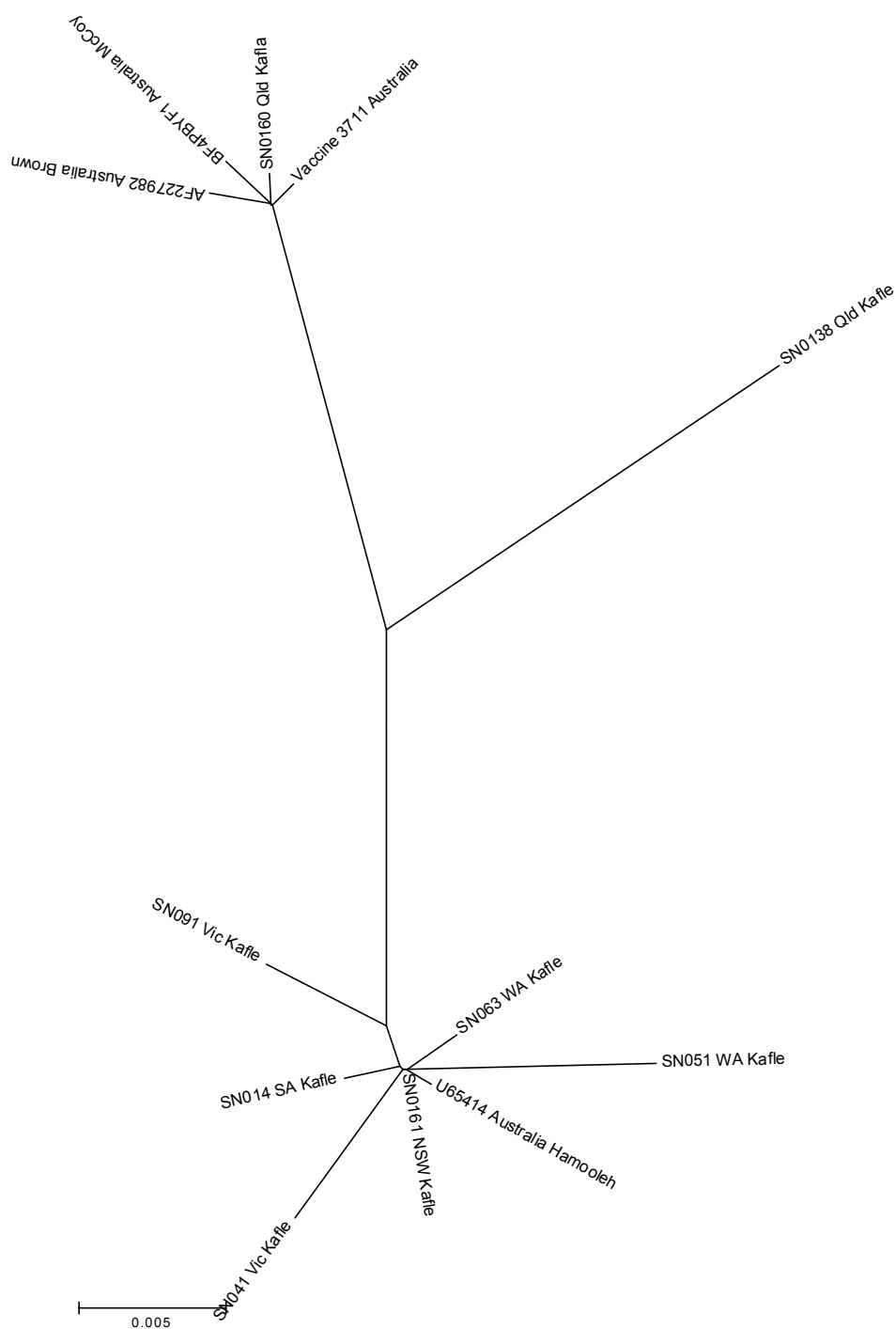
Figure 6.3 Phytogenic analysis of starting 42% sequences of VP1 Australian CAV isolates, MEGA3 (ME, tree/branch style- radiation)
