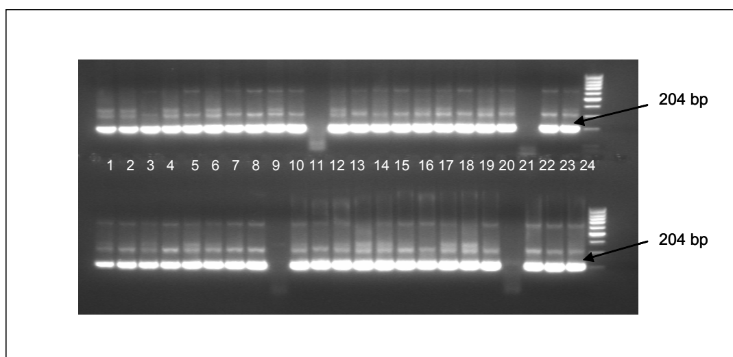
Figure 5.1 Electrophoresis of CAV nested PCR products Primers used were CAV SH-1N3 and SH-1N5 (inside primer set)
